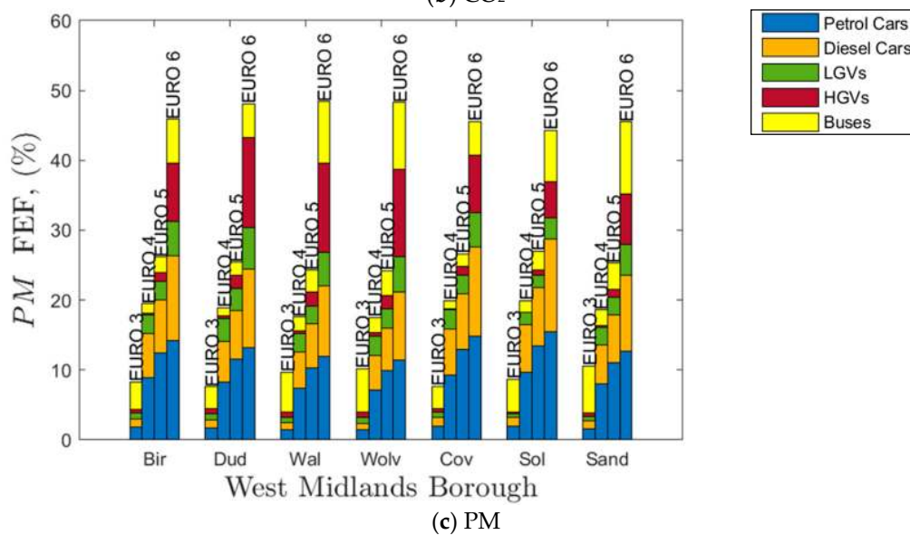
Figure 4. The effect of electrification on the percentage reduction of total fleet emissions of (a) NO_x , (b) CO_2 , and (c) PM subset by EURO class and vehicle type on urban roads, for each West Midland borough. On the y-axis, (%) is based on the total fleet emission.
