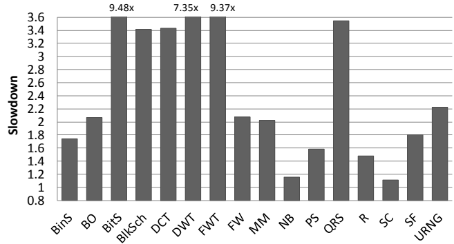
Figure 6: Performance overheads of Inter-Group RMT normalized to the runtime of the original kernel. Some kernels have extremely large slow-downs due to the high cost of communication.
