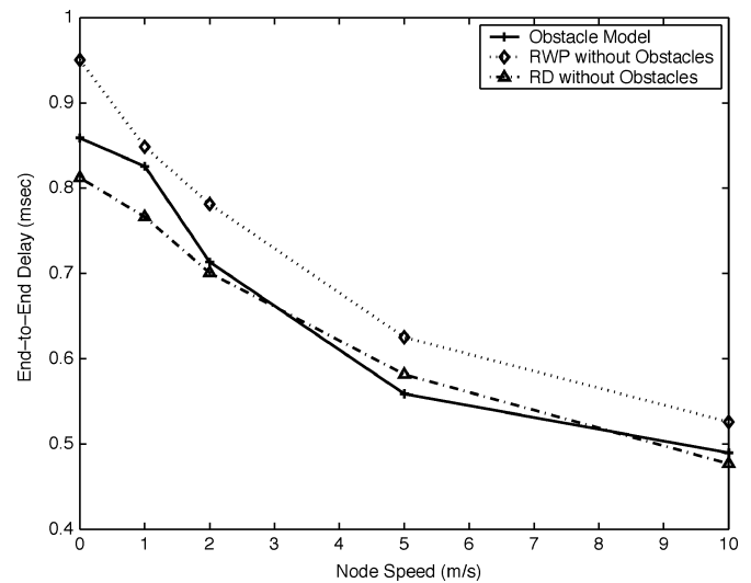
Fig. 10. End-to-end latency.
