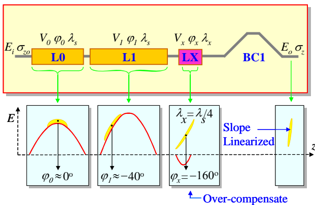
Figure 1: Schematic of two linac segments followed by harmonic RF and compressor chicane. The bunch is compressed from an initial rms length \sigma_{z0} to a final length \sigma_z with initial energy E_i and final energy E_0 (bunch head at left: z < 0 ).
