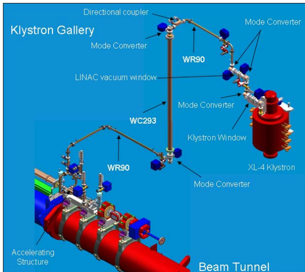
Figure 2: LCLS X-Band RF System Layout.
