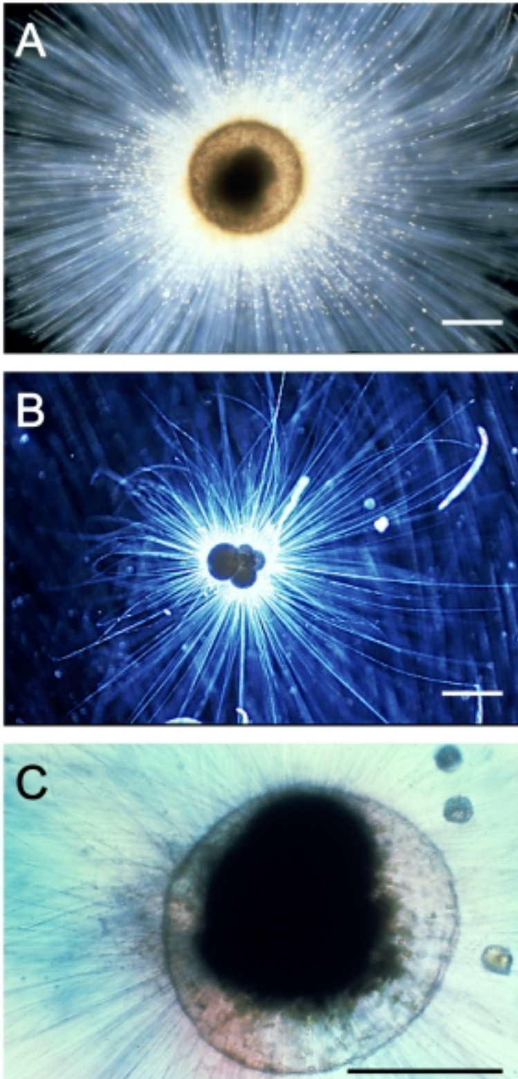
Fig. 1. Orbulina universa with symbionts (A; scale bar = 300 μm), Globigerina bulloides (B; scale bar = 300 μm), protruding membrane in O. universa (C; scale bar = 300 μm).
