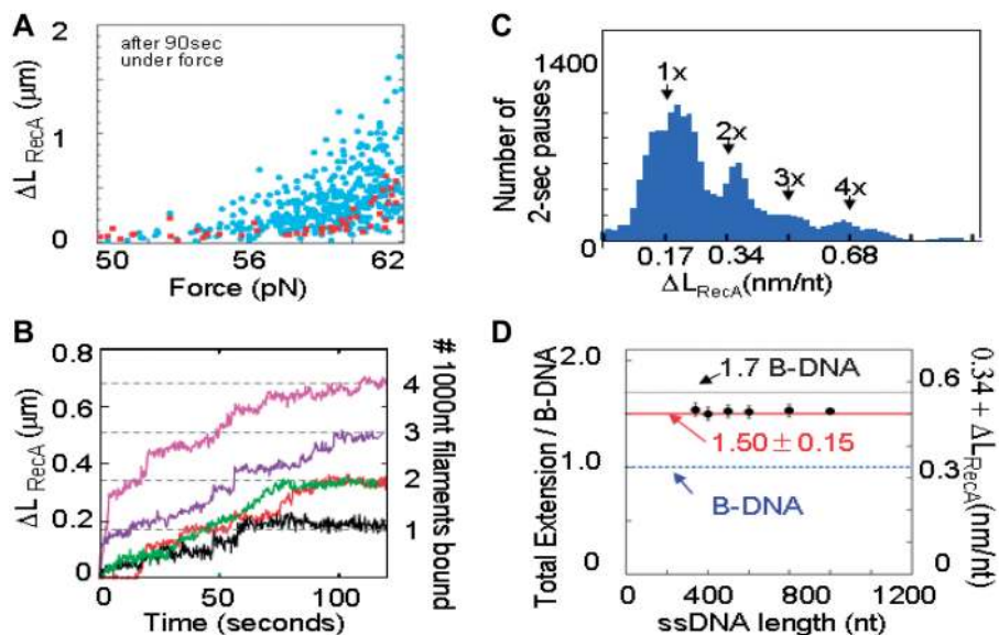
Figure 3. RecA–ssDNA filaments extend non-homologous dsDNA pulled by 3′/5′ ends. (A) \Delta L_{\text{RecA}} 's for \lambda dsDNAs controls with free ssDNA or \lambda dsDNA only (red, N = 87 ) and \lambda dsDNAs with RecA–ssDNA filaments (blue, N = 454 ). (B) Single molecule extension profiles for non-homologous binding. Different colors are used to represent the response for each different single molecule. The curves ending at positions corresponding to 1, 3 and 4 filaments are 57.0, 59.0 and 60.9 pN, respectively. The red and green curves ending at two-filament lengths correspond to 58.9 and 57.2 pN, respectively. The filaments were prepared in a buffer containing ATP \gamma S, but measured in a buffer containing ATP. Pauses at full filament lengths are indicated by horizontal bars the same color as the curve. (C) \Delta L_{\text{RecA}} probability distributions for periods of \geq 2 s constant \lambda dsDNA length, for all filaments of 400–800 nt at 50–62 pN. (D) DNA extensions within homology search complexes on dsDNA (color) or \lambda ssDNA.
