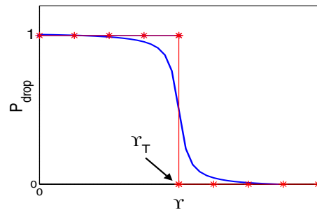
Fig. 1. Solid line: an example of packet loss probability as a function of Signal to Noise Ratio, star line: rectangular approximation
