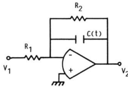
FIGURE 13. - IDEAL OPERATIONAL AMPLIFIER WITH FEEDBACK ELEMENTS.
