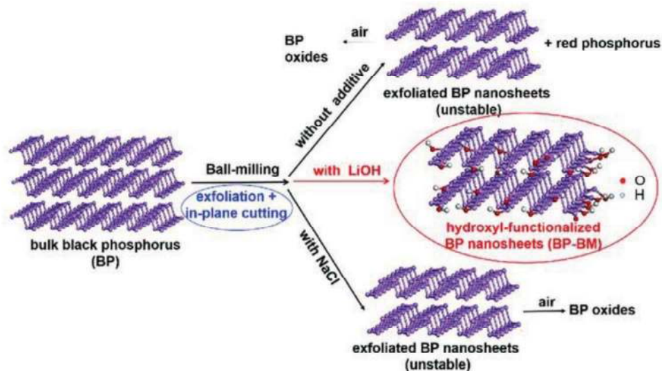
Figure 9. Scheme for the ball milling of BPNSs with additives (LiOH or NaCl) and without any additives. Reproduced with permission. [105] Copyright 2017, John Wiley and Sons.
