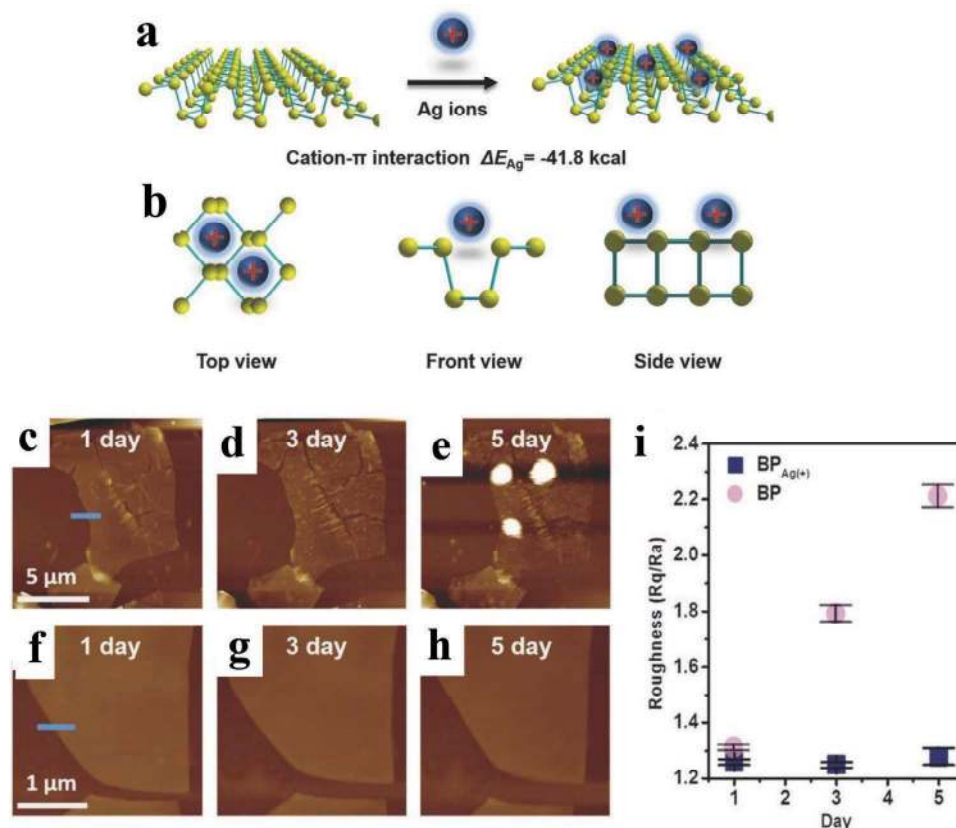
Figure 19. a) Schematic representation of adsorption of \text{Ag}^+ on BPNSs. b) Three different views of the \text{Ag}^+ -modified BPNSs. AFM images of c–e) the bare BPNSs and f–h) the \text{Ag}^+ -modified BPNSs exposed to air for 1–5 d. i) Changes in the surface roughness before and after functionalization with exposure time. Reproduced with permission. [194] Copyright 2017, John Wiley and Sons.
