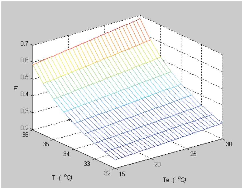
Fig. 8. The transform coefficient \eta from \Delta T_e to \Delta \omega in different temperatures
