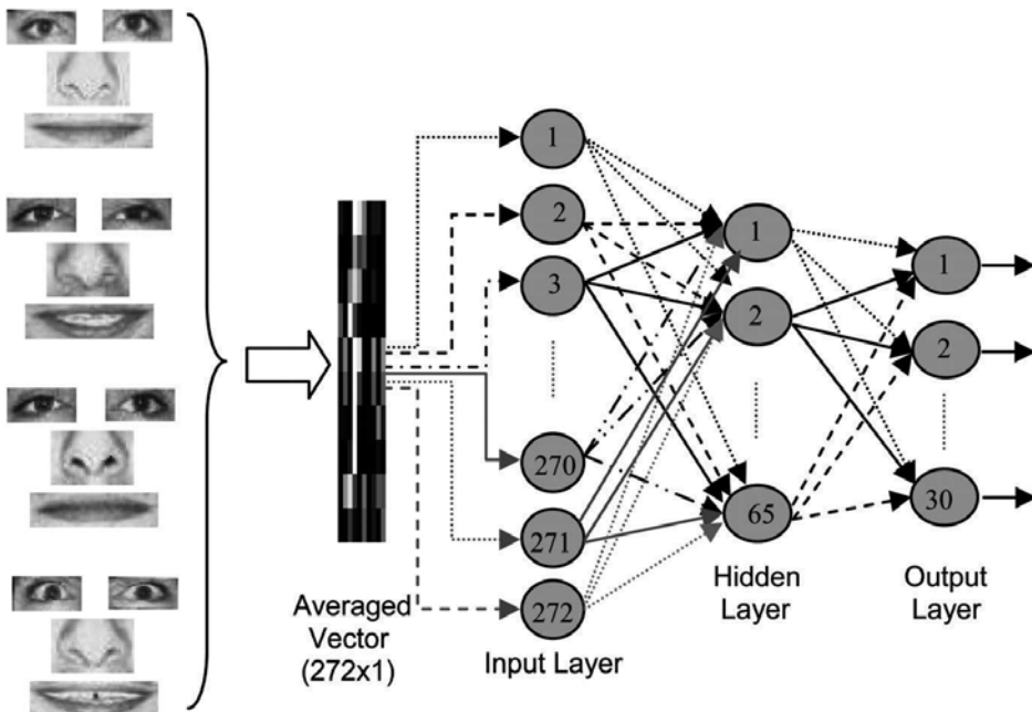
Fig. 6. Local pattern averaging and neural network design
