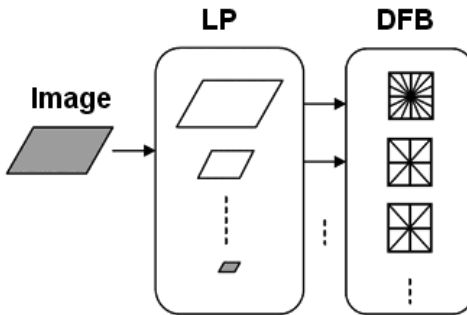
Fig. 6. Flow Filter-bank representation for Contourlets [7]
