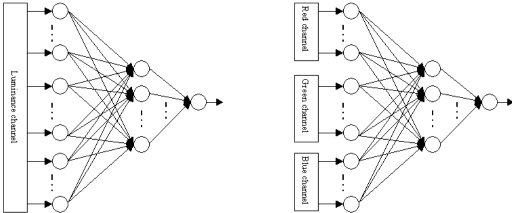
Fig. 6. Conventional v.s. proposed MLNN structures
