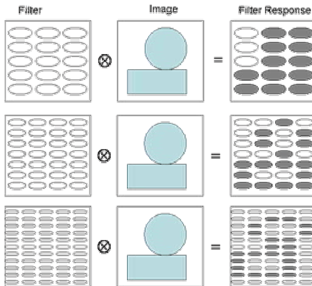
Fig. 8. Convolution of the filter-bank with an image
