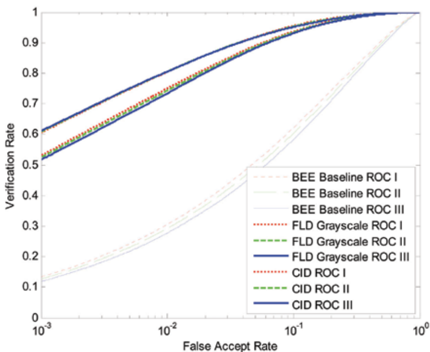
Fig. 3. ROC curves corresponding to the BEE Baseline algorithm, FLD on grayscale images and the CID Algorithm
