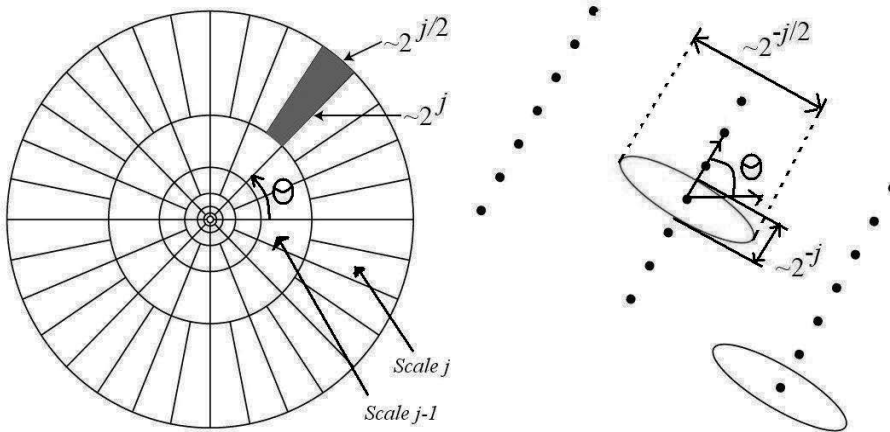
Fig. 1. Curvelet Transform: Fourier Frequency Domain partitioning (left) and Spatial Domain representation of a wedge (right) [4]
