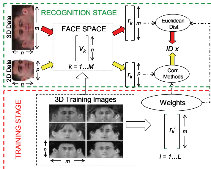
Fig. 5. General Block Diagram of P 2 CA Approach
