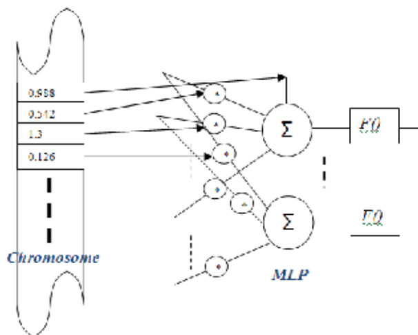
Fig. 8. Weight/bias mapping
