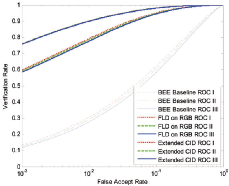
Fig. 7. ROC curves corresponding to the BEE baseline algorithm, FLD using the RGB images, and the extended CID algorithm (for three color components) using the decision-level fusion strategy
