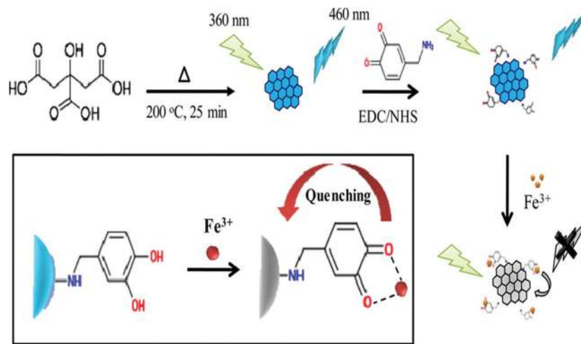
Fig. 7 Surface functionalization of GQDs with DA using EDC/NHS chemistry by activating the -\text{COOH} groups of GQDs and coupling with the -\text{NH}_2 groups of DA (reproduced with permission from ref. 162, copyright 2016 American Chemical Society).
