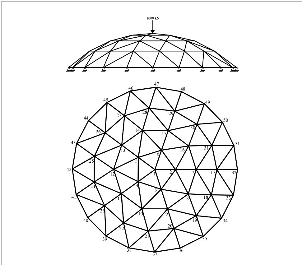
Fig. 4. Geodesic dome
