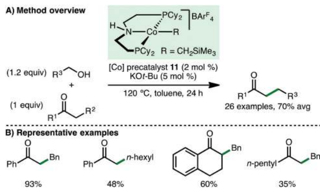
Scheme 19 Co-Catalysed \alpha -alkylation of ketones (Zhang).
