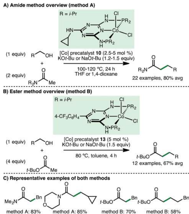
Scheme 18 Co-Catalysed \alpha -alkylation of unactivated amides and esters (Kempe).
