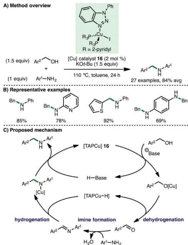
Scheme 28 Cu-Catalysed N -alkylation of arylamines (Wang).
