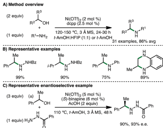
Scheme 27 Ni-Catalysed N -alkylation of using secondary alcohols (Tang, Zhou).
