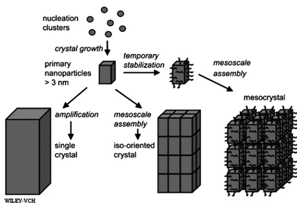
Fig. 2 Schematic representation of classical and aggregation-based crystallization. (Left) Classical crystallization pathway (a), (centre) oriented attachment of primary nanoparticles forming an iso-oriented crystal upon fusing (path (b)), (right) mesocrystal formation via self-assembly of primary nanoparticles covered with organics (path (c)). From ref. 57. Copyright © 2005 Wiley-VCH.
