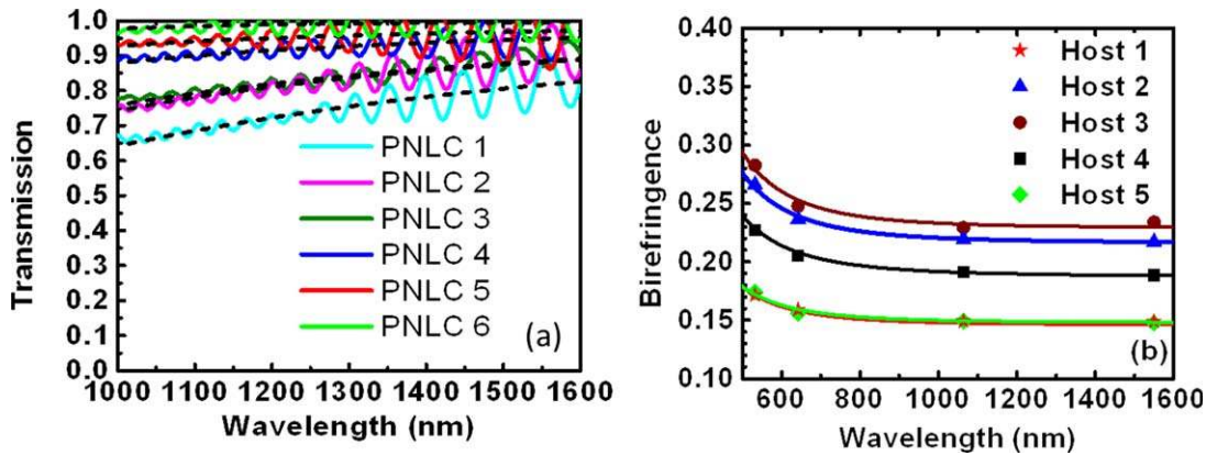
FIGURE 8 (a) Transmission spectra of PNLC 1–6 with V_{max} applied. Solid lines: experimental results; dashed lines: fitting results with eq 8. (b) Wavelength-dependent \Delta n of the five LC hosts.
