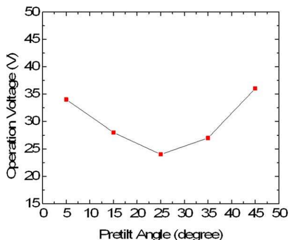
FIGURE 18 Simulated pretilt angle effect on the operating voltage of PNLC cells at \lambda = 633 nm for 2\pi phase change in reflective mode. Cell gap d = 5 \mu\text{m} , \Delta\epsilon = 86 , and \Delta n = 0.3 .
