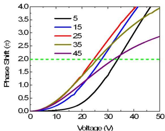
FIGURE 17 Simulated pretilt angle effect on the phase change of PNLCs in reflective mode at \lambda = 633 nm. Cell gap d = 5 \mu\text{m} , \Delta\epsilon = 86 , and \Delta n = 0.3 .
