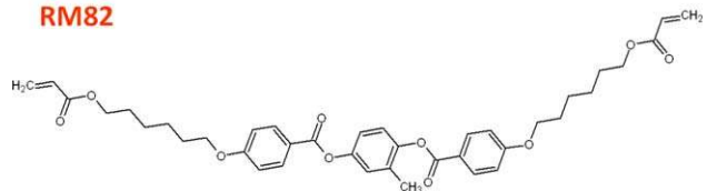
FIGURE 5 Examples of di-functional monomers used in PNLC.
