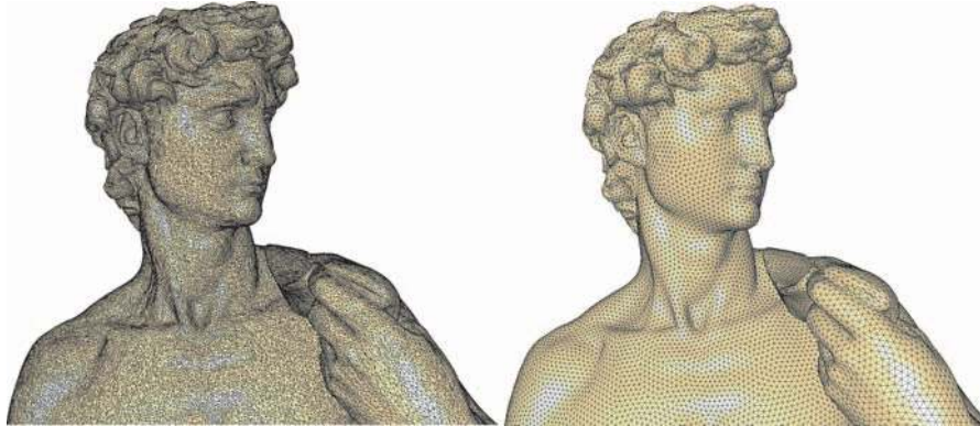
Fig. 1. Uniform remeshing of the Digital Michelangelo David model. Figure reproduced from [78].
