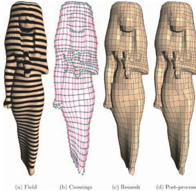
Fig. 11. Quadrilateral remeshing of arbitrary manifolds: (a) A harmonic function is computed over the manifold. (b) A set of crossings along each flow line is constructed. (c) A non-conforming mesh is extracted from this net of flow crossings. (d) A post-process produces a conforming mesh composed solely of triangles and quadrilaterals. Figure reproduced from [18].
