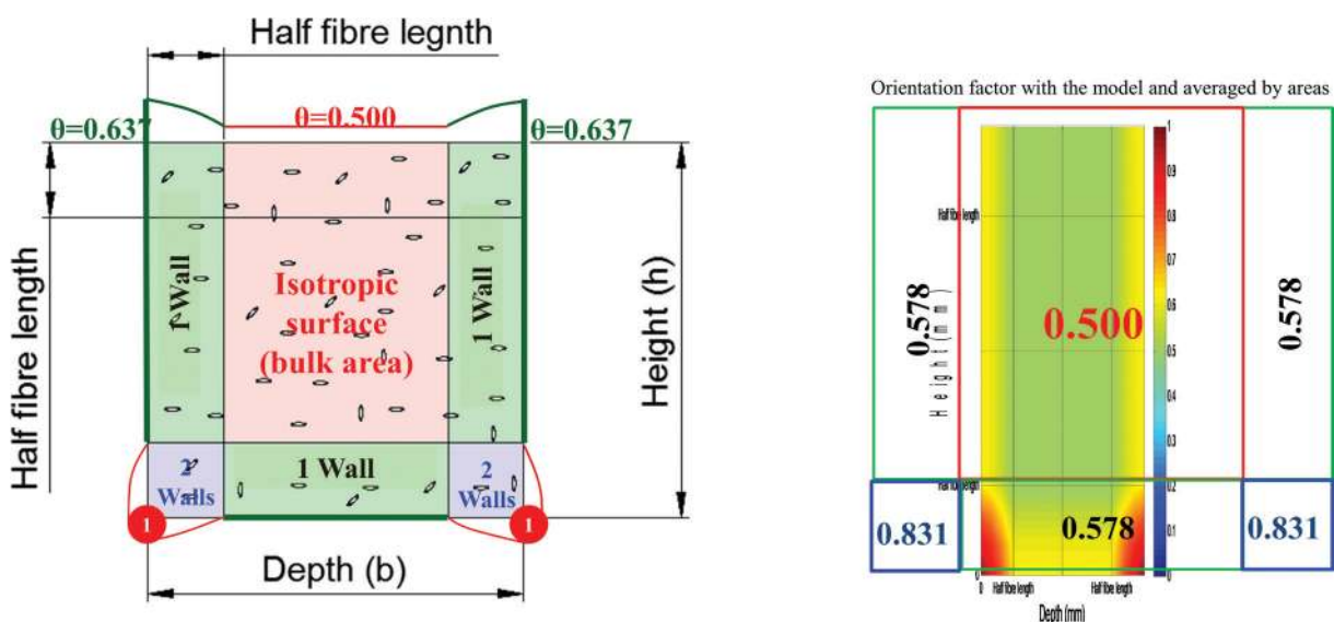
FIGURE 19. Probability distributions in a rectangular section (31).
