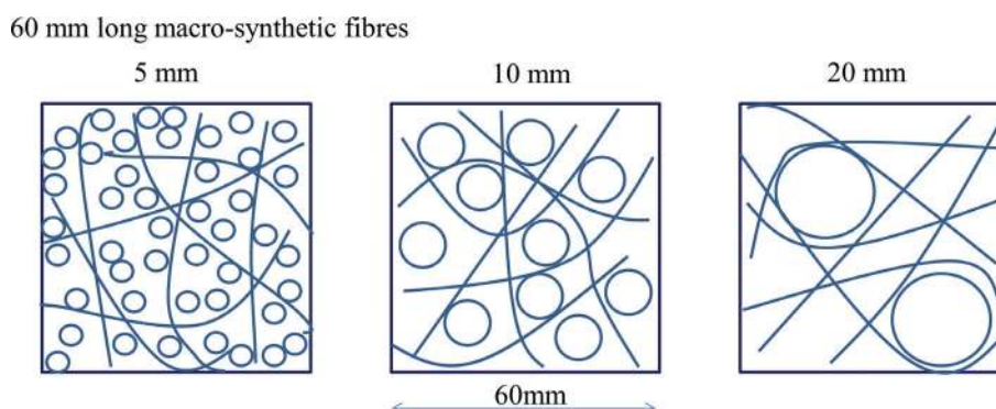
FIGURE 2. Effect of the aggregate size on the fibre distribution (31).
