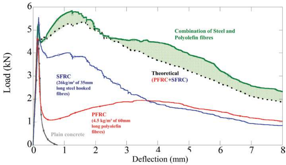
FIGURE 25. Fracture results of the combination of steel hooked fibres and polyolefin fibre and the sum of the residual contributions of mono-fibre-reinforced mixtures. Adapted from: (40).
