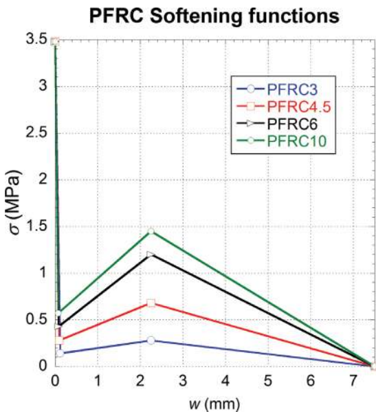
FIGURE 29. Softening functions (left) and comparison among simulated and experimental results (right). Adapted from: (100).
