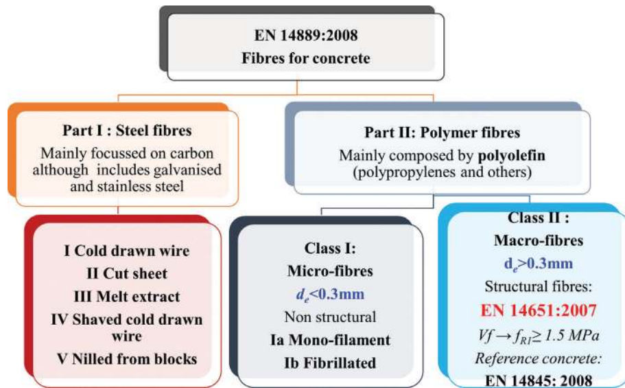
FIGURE 1. Fibre classification following EN-14889. Adapted from: (43).
