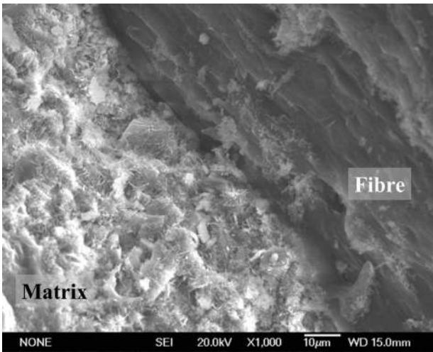
FIGURE 13. Interface between polyolefin fibre and cement paste (69). Adapted from: (31, 69).
