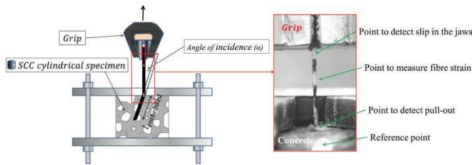
FIGURE 11. Sketch of the test configuration, using concrete specimens and points used to obtain slip, strain or fibre slip inside the jaws. Adapted from: (31, 69).
