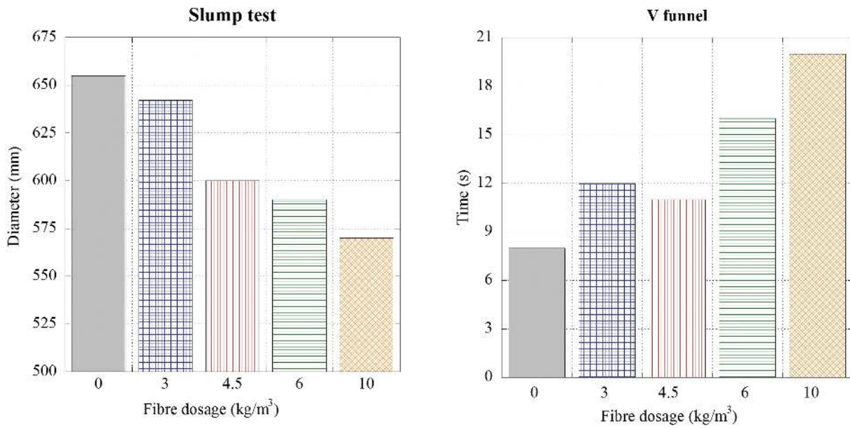
FIGURE 3. Slump-flow and V-funnel test results in a PFRC-SCC. Adapted from: (31).
