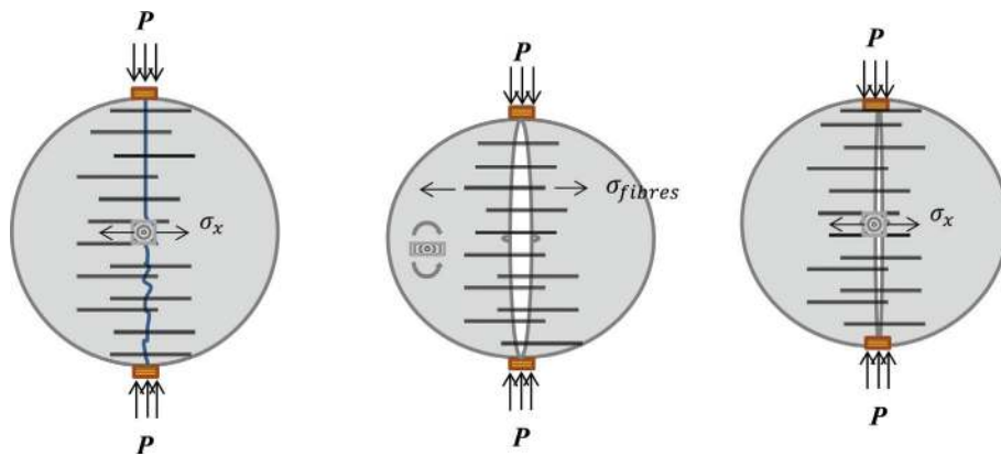
FIGURE 7. Second order effects during indirect tensile strength tests with FRC (31).
