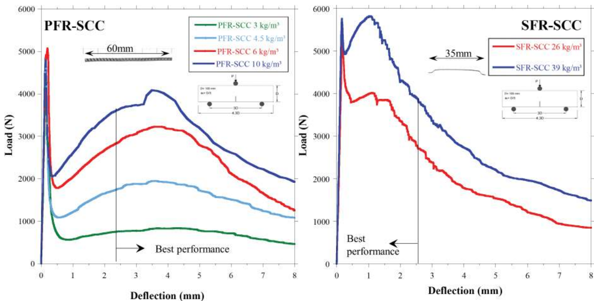
FIGURE 24. Sketch of the best performance of each fibre type. Adapted from: (81).
