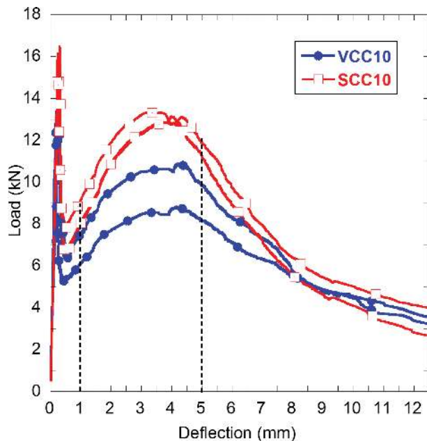
FIGURE 18. Load-deflection curves obtained in fracture tests of VCC and SCC with 10kg/m 3 of polyolefin fibres (27).
