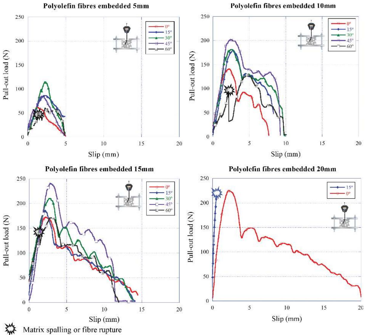
FIGURE 12. Influence of the inclining angle of polyolefin fibres embedded in a SCC (69).Adapted from: (31, 69).
