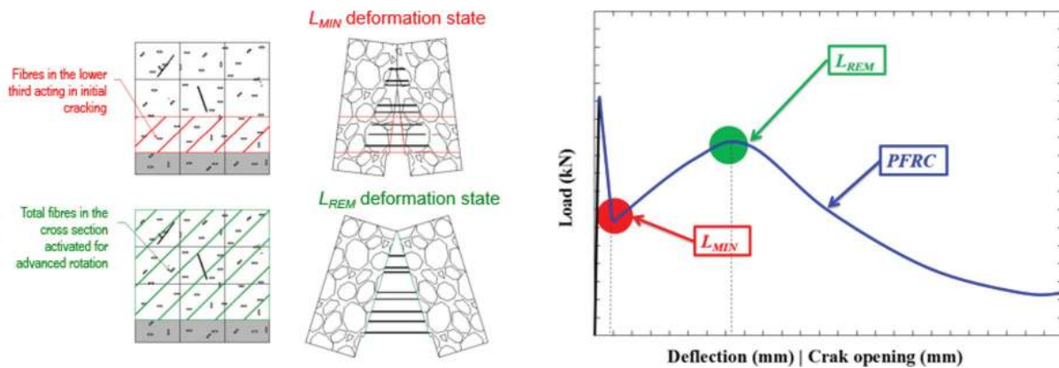
FIGURE 17. Deformation states of SLS or ULS. Adapted from: (31, 41).
