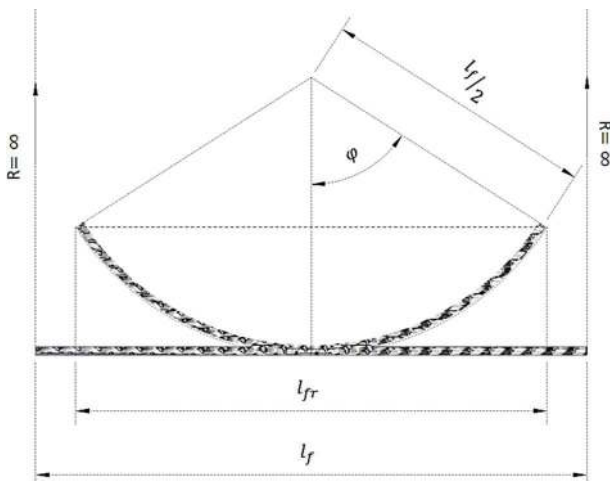
FIGURE 21. Fibre bending and reduction of its mean projection (31).
