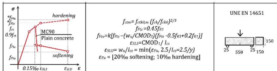
FIGURE 27. Constitutive models and tests of MC2010. Adapted from: (85).
