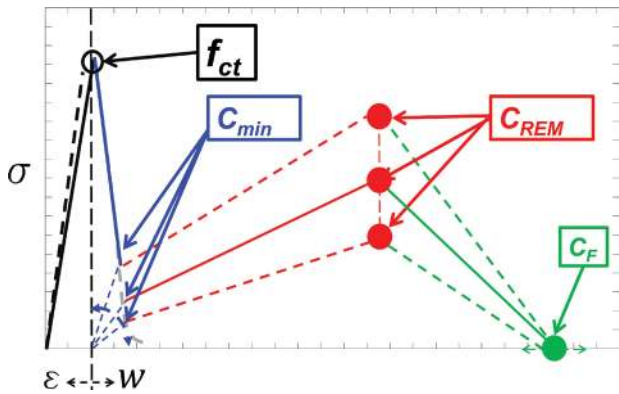
FIGURE 30. Scheme of the constitutive relations for PFRC (31).
