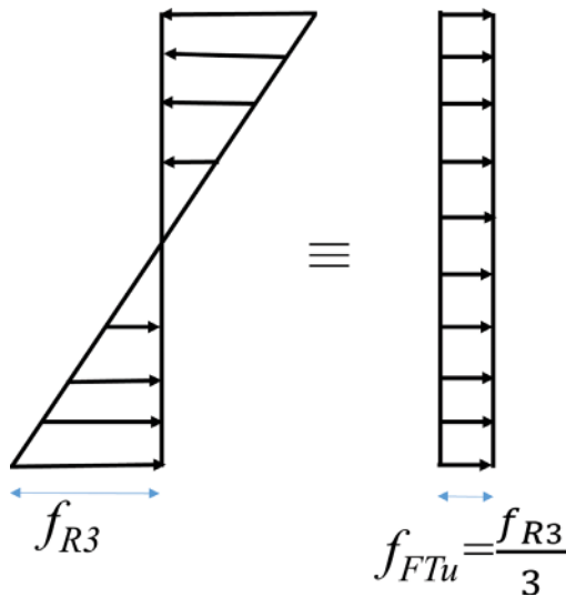
FIGURE 28. Simplified model adopted to compute the ultimate residual tensile. Adapted from: (16).
