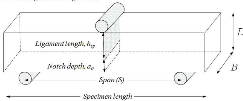
Three-point bending tests configuration
