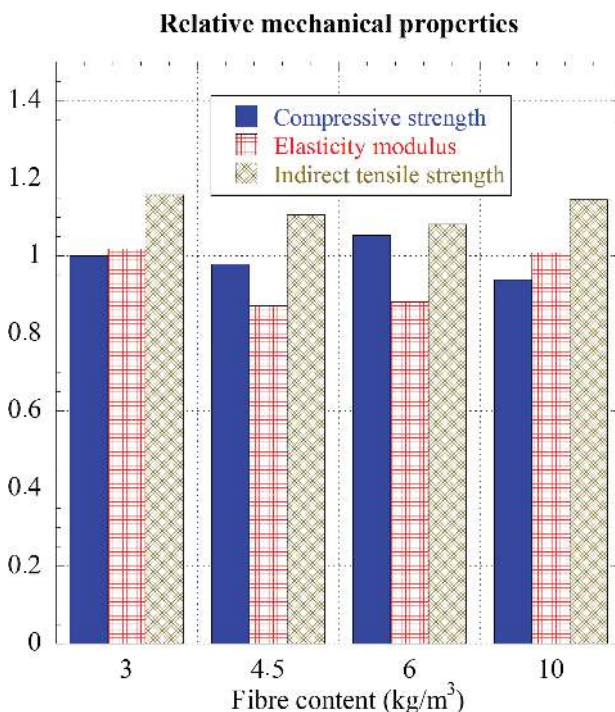
FIGURE 8. Mechanical properties of PFRC with respect to plain concrete which is taken as the unity values. Adapted from: (31, 41)
