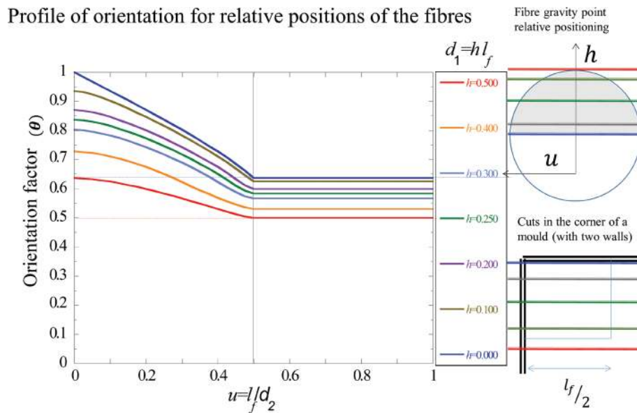
FIGURE 20. Profile of the value of the orientation factor as a function of the distance between fibre gravity point and the each of the two walls (31).
