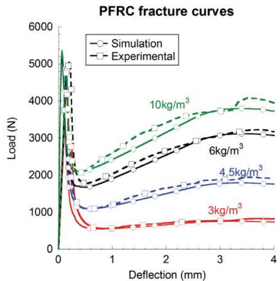
FIGURE 29. Softening functions (left) and comparison among simulated and experimental results (right). Adapted from: (100).
