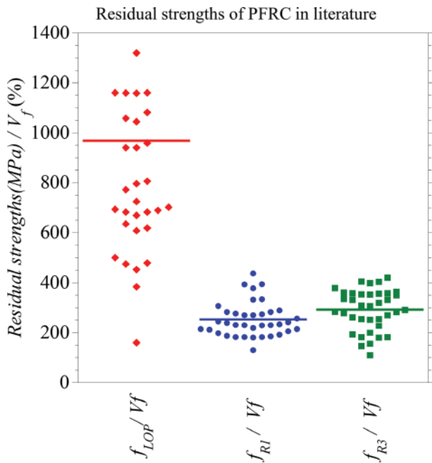
FIGURE 23. Representative values of the relation of strengths and volume fraction ( f_{LOP}/V_f , f_{RI}/V_f and f_{R3}/V_f ) of macro-synthetic fibres found in the literature.
