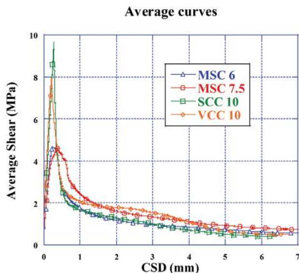
FIGURE 32. Average curves CSD vs. average shear ( \tau_{aver} ) of the four types of concrete (107). The figure shows the results obtained with a medium-strength concrete with 6 and 7.5kg/m 3 of polyolefin fibres (MSC6 and MSC7.5), a conventional vibrated concrete with 10kg/m 3 (VCC10) of polyolefin fibres and a self-compacting concrete with 10kg/m 3 of polyolefin fibres.
