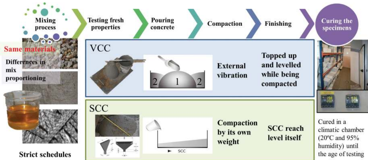
FIGURE 6. Typical concrete production procedures for VCC and SCC (31).
