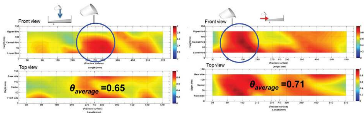
FIGURE 5. Variation of the orientation factor in standard specimens by filling the moulds with PFRC self-compacting concrete from: (a) the centre; (b) one side. Adapted from: (26).
