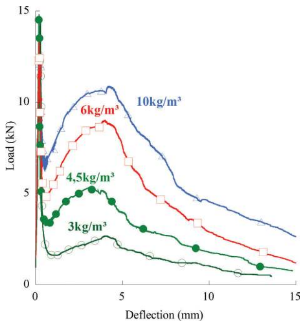
FIGURE 15. Fracture behaviour of PFRC with several contents of fibres. Adapted from: (31).
