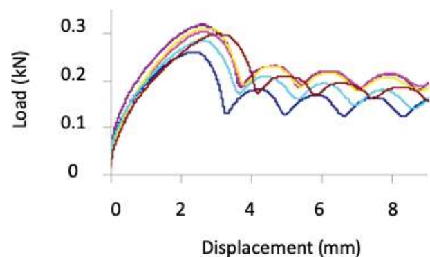
FIGURE 10. Pull-out test of a polyolefin based macro-fibre made by Døssland. Adapted from: (67).
