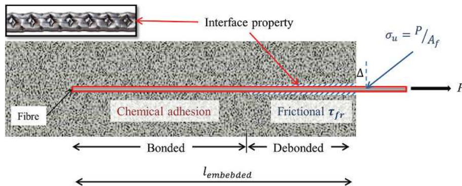
FIGURE 9. Pull-out mechanisms (31).
