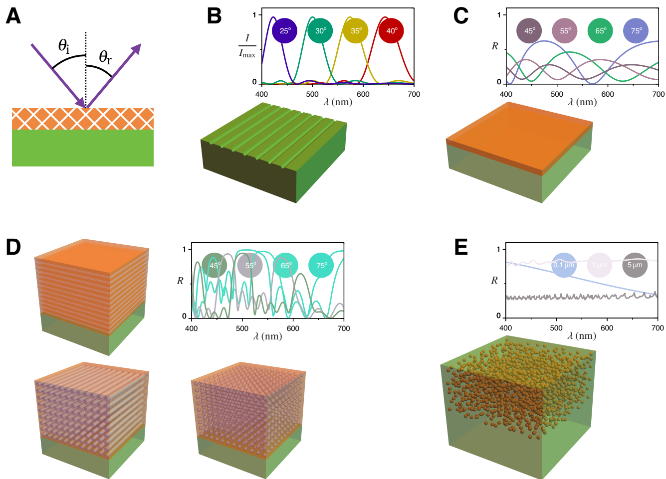
Fig. 1 (A) The reflectance of a colour-producing structure, in contact with the incident medium and supported by a substrate, must be assessed for given incidence and reflection angles, \theta_i and \theta_r , respectively; specular reflection is for \theta_i = \theta_r . (B) A reflective diffraction grating is obtained when a reflecting surface displays periodic patterns: here, parallel grooves are etched at regular intervals; the inset gives a typical spectrum of reflected intensity, showing angle-dependent wavelength discrimination. (C) Colouration can be obtained when a thin film of material is deposited on a substrate; the inset shows a corresponding example of reflectance spectrum at different angles of specular reflection. (D) One-, two- and three-dimensional (1D, 2D and 3D) photonic crystals have a structural periodicity in one, two, or three directions, respectively; in principle, photonic crystals are considered infinite, but in practice, they are bounded by a substrate and the exterior. 1D photonic crystals are multi-layers stacks, and the inset gives a typical spectrum of their reflectance. (E) Light scattered by a slab of a turbid material is also a kind of structural colour; for sufficiently small scatterers, the reflected spectrum favors lower wavelengths (blue) as illustrated by the spectra shown in inset for various scatterers' sizes.
