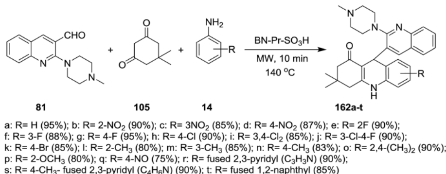
Scheme 56 Synthesis of piperazinyl-quinoliny-acridinone systems.
