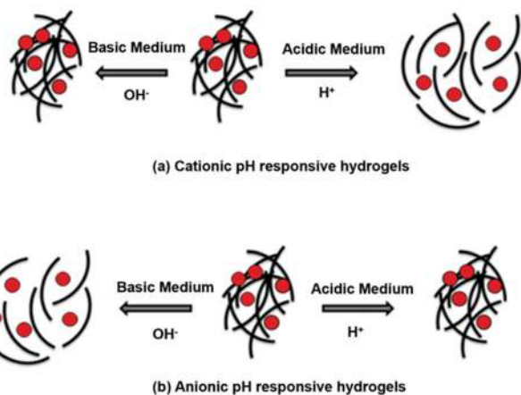
Fig. 14 The schematic representation of pH-responsive hydrogels. (a) Cationic hydrogels swell at low pH and deswell at high pH. (b) Anionic hydrogels swell at high pH and deswell at low pH [reprinted with permission from ref. 190, ©2019 by the authors, open access under attribution 4.0 international (CC BY 4.0)].
