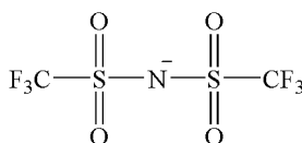
Bis(trifluoromethylsulfonyl)imide, [NTf_2]^-
