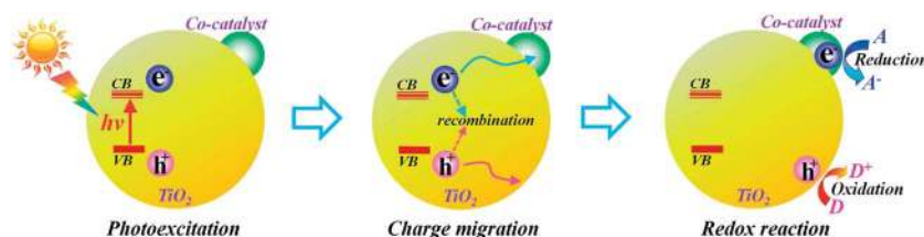
Fig. 2 Schematic picture of the \text{TiO}_2 photocatalytic reaction process.
