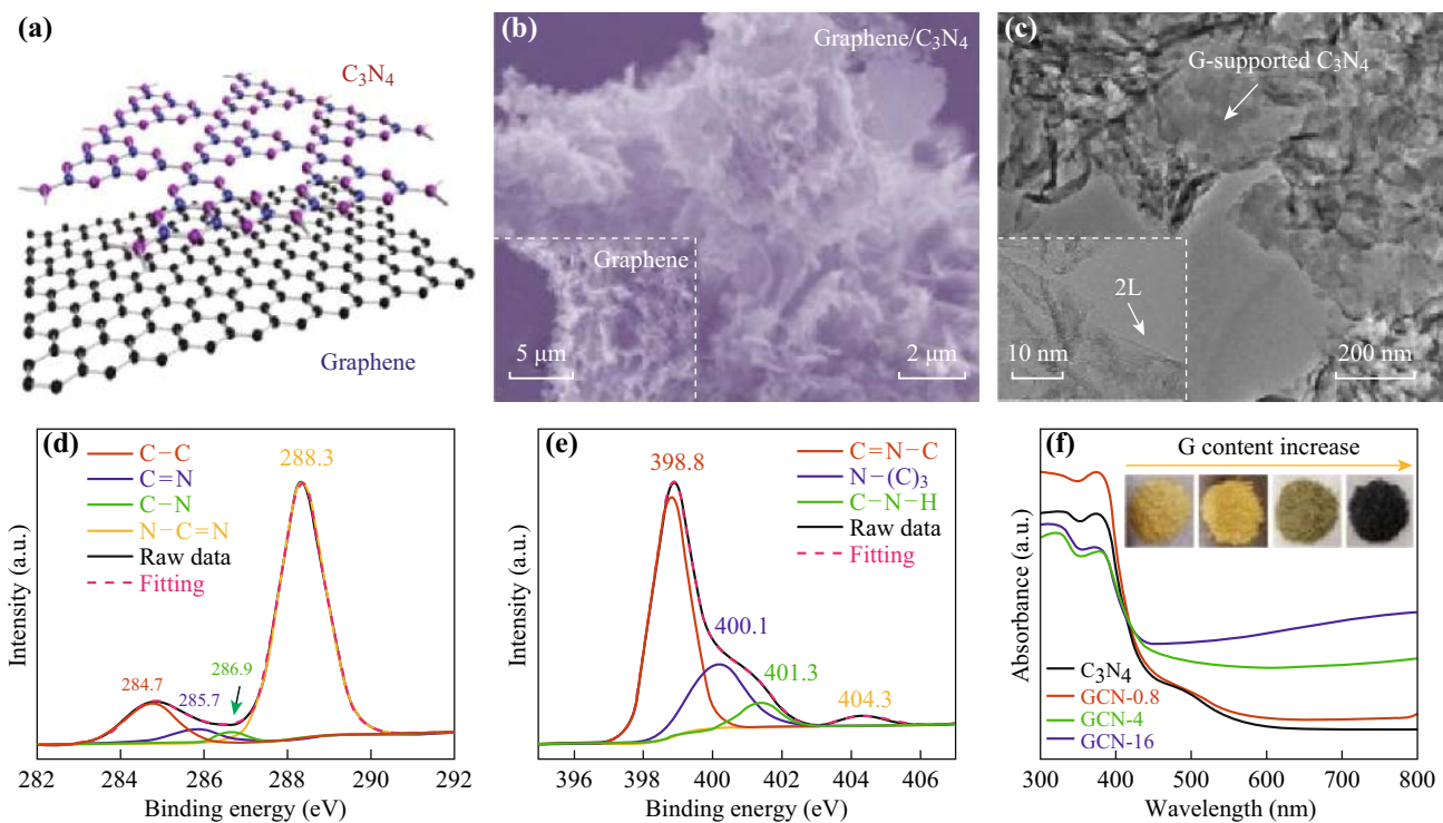
Fig. 3 a Schematic 3D g-C 3 N 4 /Graphene structures. b , c SEM images of g-C 3 N 4 /graphene nanocomposites. Inset TEM image. d C 1s, e N 1s XPS and f UV-vis spectra of g-C 3 N 4 /graphene nanocomposites. Insets : photographs of the powder samples. Reprinted with permission from Ref. [66]. Copyright 2016 American Chemical Society
