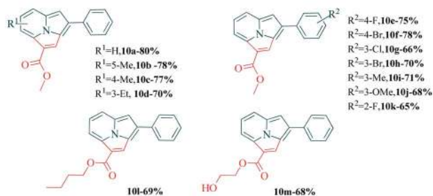
Scheme 3 Rose Bengal catalyzed intermolecular [3 + 2] alkenylation-cyclization.
