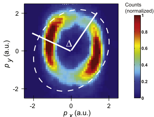
Fig. 6. Momentum distribution arising from close-to-circularly polarized laser pulses. The polarization ellipse is depicted by the white dashed line. The white solid lines indicate the maxima of the polarization ellipse and the ion momentum distribution. Adapted from [24].
