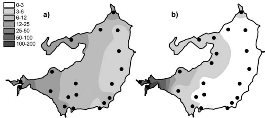
Figure 3 Spatial distribution of average chlorophyll concentration ( \mu\text{g}/\ell ) in the 0 to 5 m stratum in Albert Falls Dam in October 2006 (a) and January 2007 (b). Points correspond to sampling stations numbered in Fig. 1.
