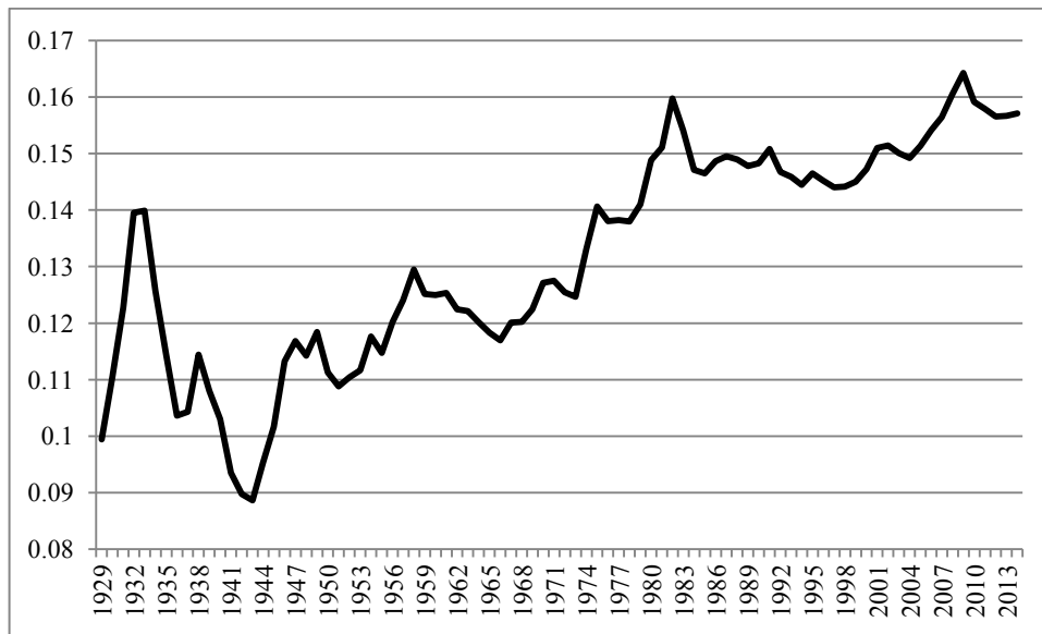
Figure 3: Depreciation/GDP
