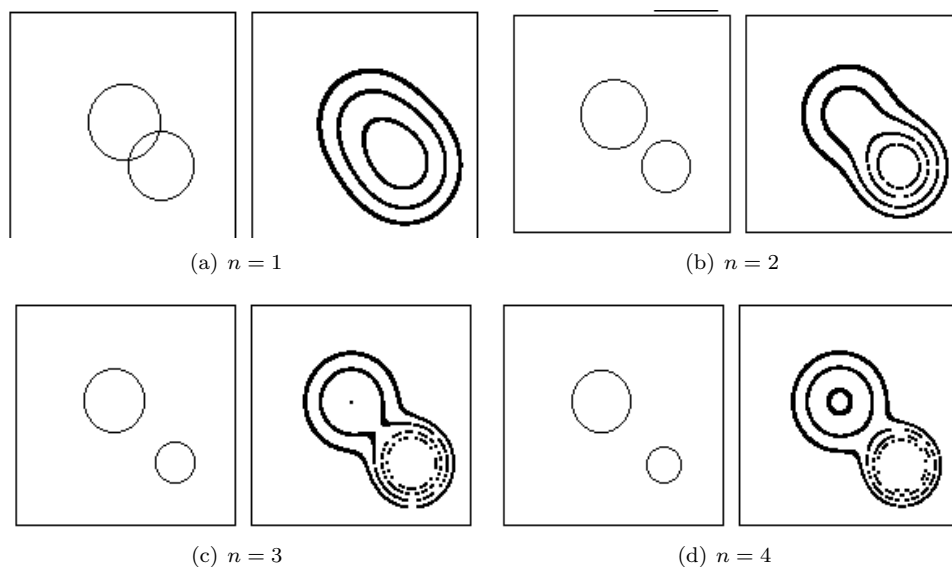
Figure 4: The em algorithm after n iterations. An insightful view of the algorithm is to think of it in terms of lower-bound estimation: at each iteration, a “tighter” lower bound is computed, and the cluster estimates “climb” closer to the (unknown) true distribution.
