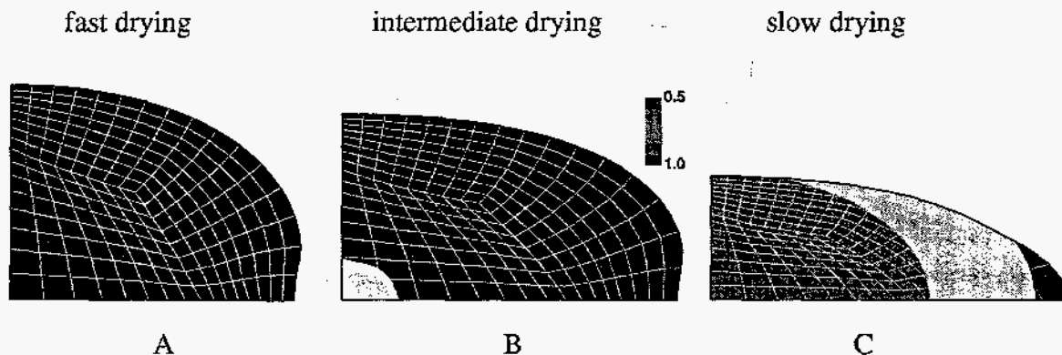
Figure 4 Finite element models of 58 vol% slurries that have been dried for five minutes at: A) fast drying rate, k = 0.001 cm/s, B) intermediate drying rate, k = 0.0001 cm/s, and C) slow drying rate, 0.00001 cm/s. The color scale represents the slurry viscosity throughout the grid. A viscosity of 1.0 indicates that the slurry has become dilatant.
