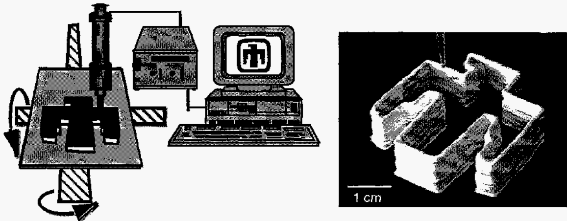
Figure 1. Schematic of the Robocasting process with an inset photo of an aluminum oxide thunderbird made in 20 layers and sintered crack-free to 96% theoretical density.
