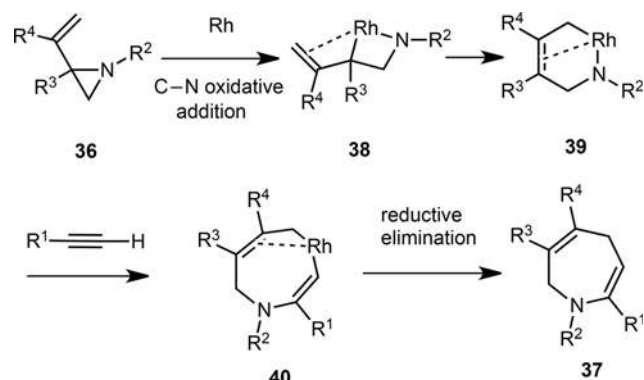
Scheme 13. Mechanism for rhodium-catalyzed intermolecular hetero [5+2] cycloaddition of vinylaziridines and alkynes.
