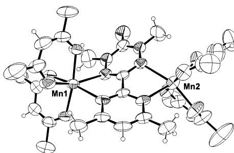
Fig. 4 Molecular structure of (\text{hfac})_2\text{Mn}27\text{Mn}(\text{hfac})_2 .
