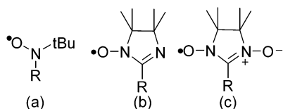
Scheme 1 General structures of nitroxide (a), imino nitroxide (b), and nitronyl nitroxide (c) free radicals.
