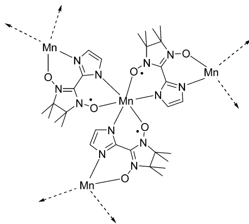
Fig. 2 Schematic of a unit of the two-dimensional layered structure of 13 .
