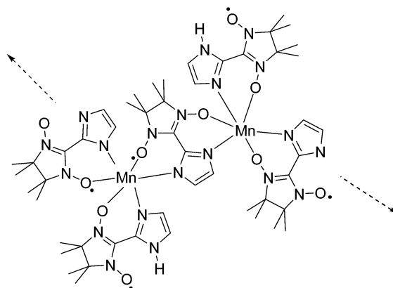
Fig. 1 Schematic of a fragment of the one-dimensional chain 12 .
