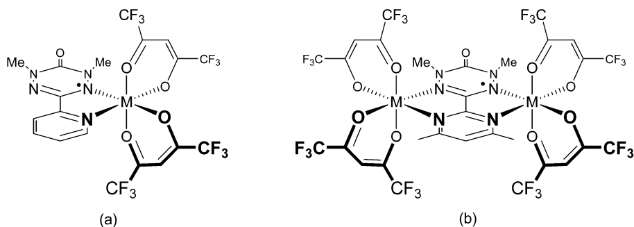
Scheme 5 M(\text{hfac})_2 ( M = \text{Mn}, \text{Ni} ) complexes with verdazyl 25 (a), and bimetallic complexes with verdazyl 27 (b).
