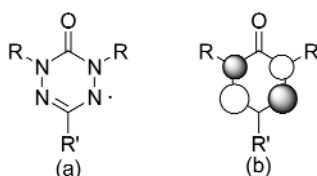
Scheme 2 General structure (a) and \pi -SOMO of a 6-oxo-verdazyl radical.
