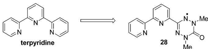
Scheme 6 Structural relationship between verdazyl 28 and terpyridine.
