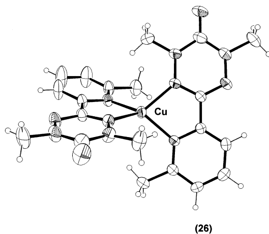
Fig. 3 Molecular structure of a copper(I) complex containing verdazyl 26 .
