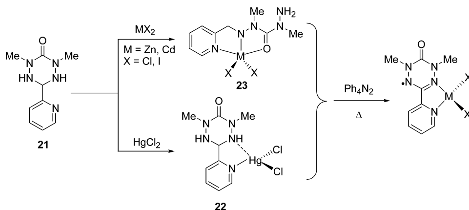
Scheme 4 Reaction of 21 with group 12 metal halides, and subsequent oxidation with tetraphenylhydrazine to generate metal-radical complexes.
