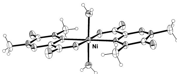
Fig. 6 Molecular structure of Ni( 29 ) 2 (H 2 O) 2 .
