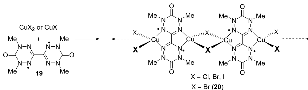
Scheme 3 Preparation of one-dimensional polymers of 19 with copper halides.
