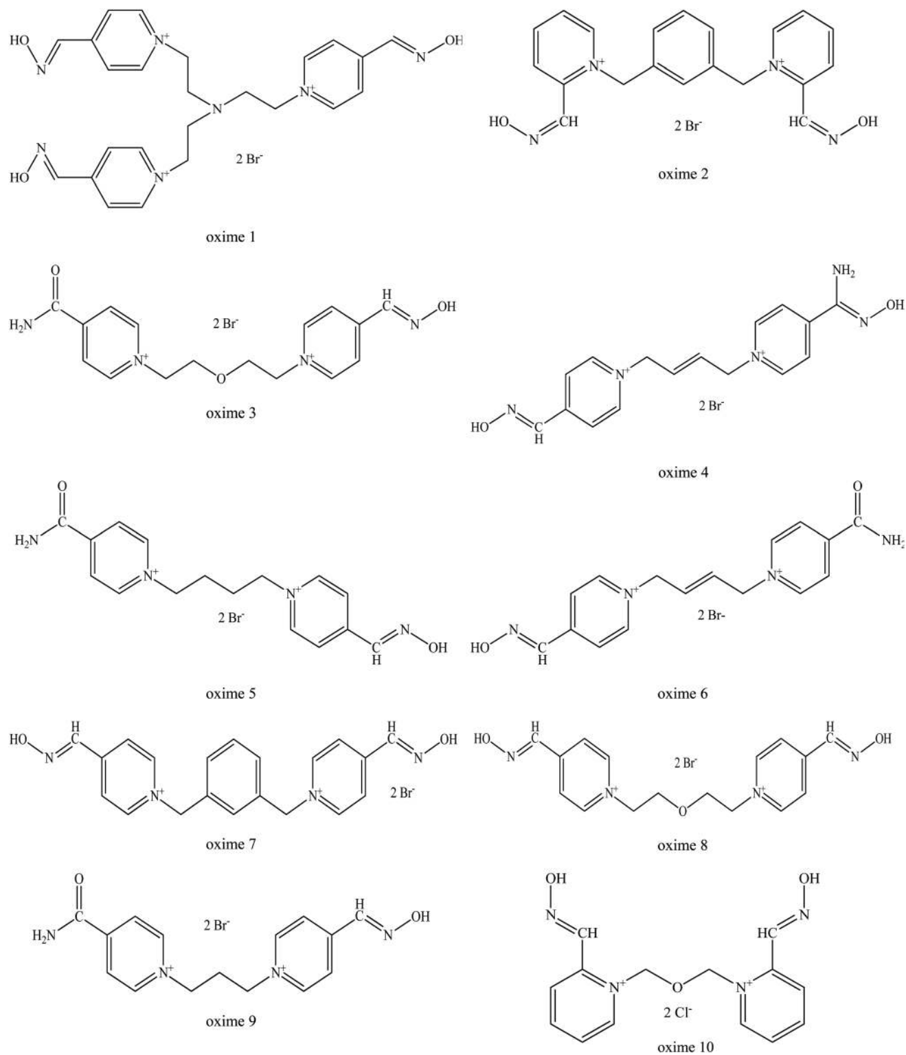
Fig. 6 List of oximes as reported by Karsova et al. (2010). 63
