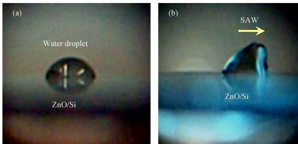
Fig. 6. A 2 μl water droplet in (a) and its movement along with the propagating acoustic wave in (b) showing the droplet is pushing upward and forward.
