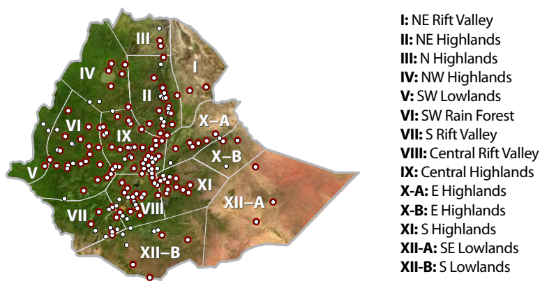
Figure 1 Precipitation zones and stations
