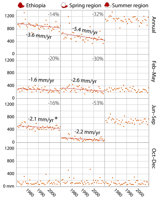
Figure 10 Precipitation trends
