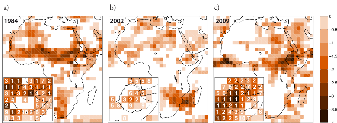
Figure 8 Continental SPI distribution in 1984, 2002 and 2009
