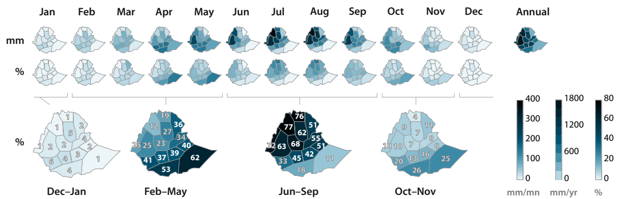
Figure 3 The seasonal precipitation cycle in Ethiopian rainfall zones
