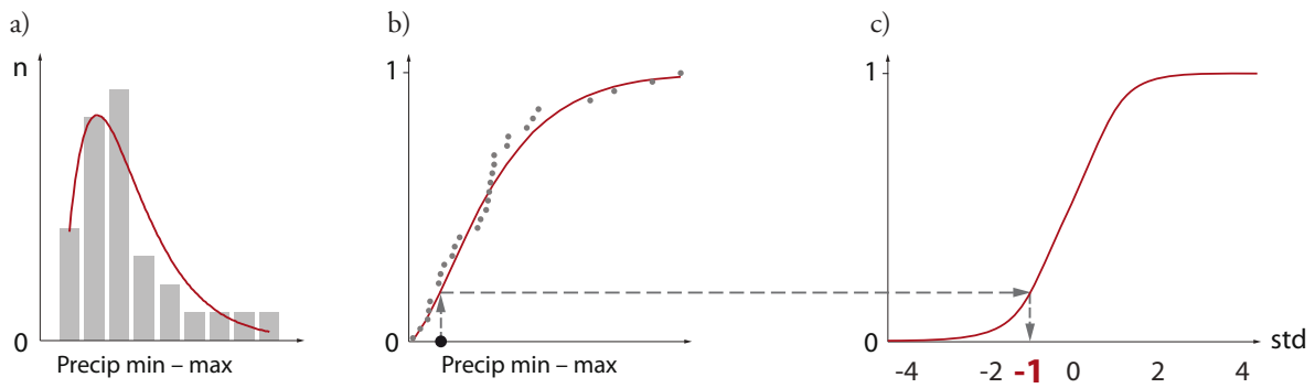
Figure 2 Calculating the Standardized Precipitation Index (SPI)
