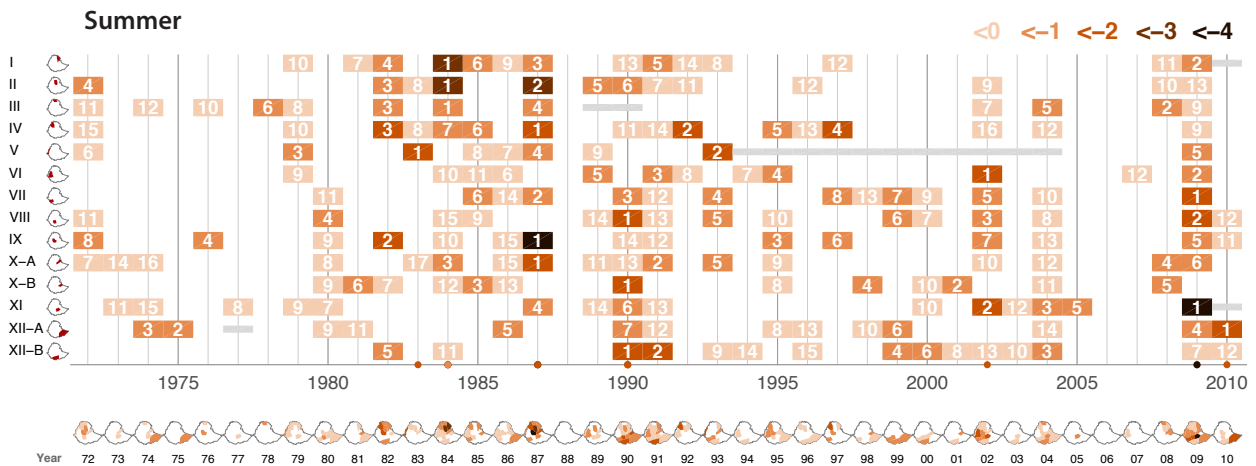
Figure 4 Annual SPI and rank (upper)
