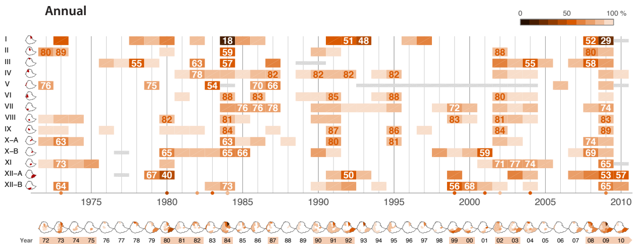
Figure 7 Percentage of mean annual precipitation
