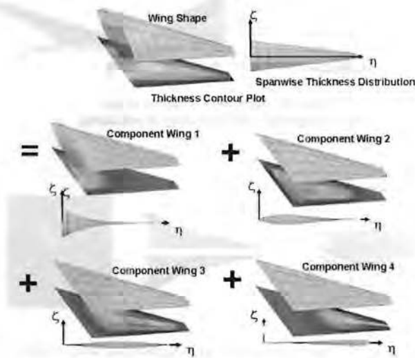
Figure 35. Example of BP03 spanwise analytic wing components.
