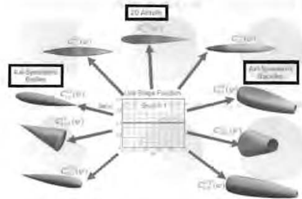
Figure 11. Geometries derivable from a unit shape function.
