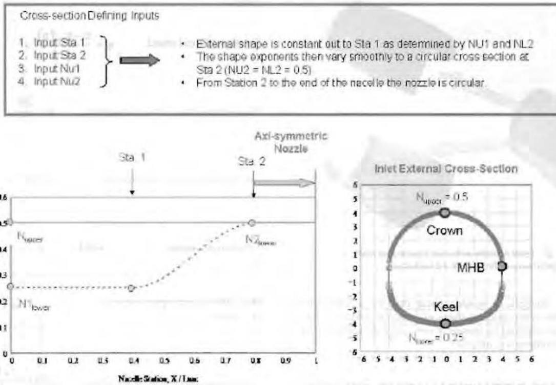
Figure 23. Nacelle shape distribution circumferentially around the nacelle centerline \rightarrow four variables.
