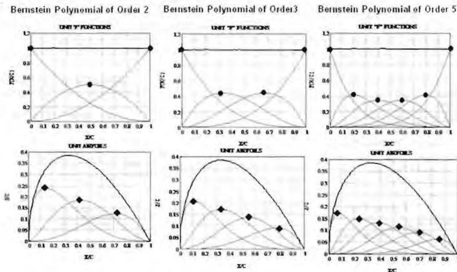
Figure 7. Bernstein polynomial provides 'natural shapes'.
