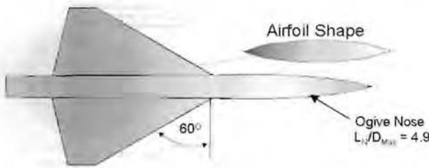
Figure 34. Basic delta wing/body.
