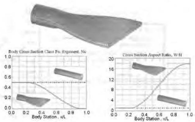
Figure 20. Two variable transformation of a circular duct to a thin rectangular nozzle.
