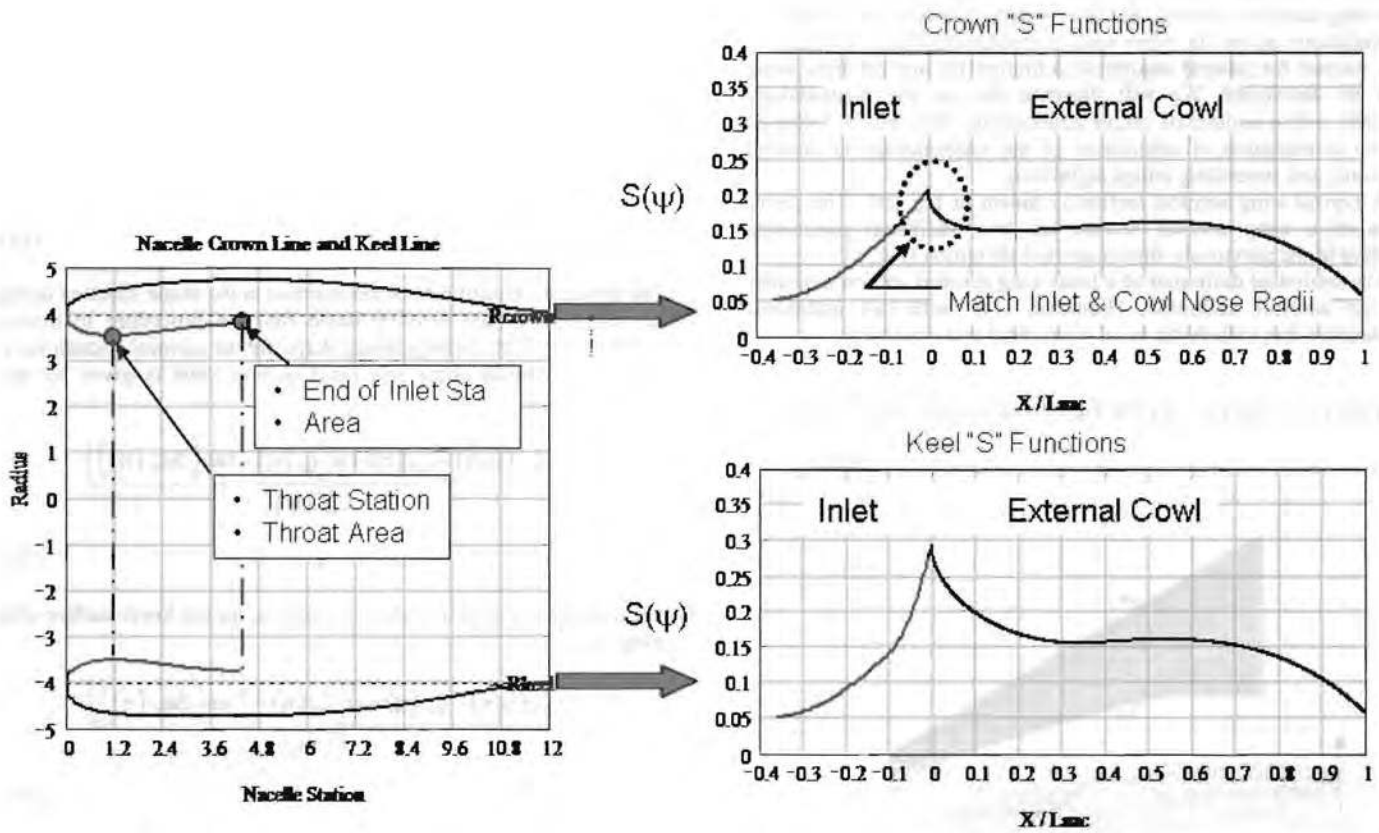
Figure 24. Nacelle inlet geometry definition \rightarrow 4 variables.
