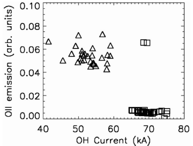
Figure 6. Oxygen II emission at the centrestack for plasmas limited by the stainless steel tray ( \Delta ) and by liquid lithium ( \square ).
