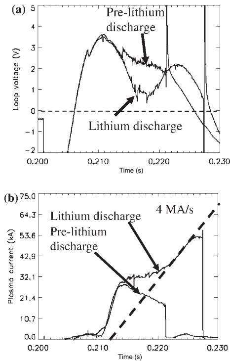
Figure 5. Loop voltage (a) and plasma current (b) comparison for pre- and post-lithium discharges. Note the zero in the loop voltage plot.
