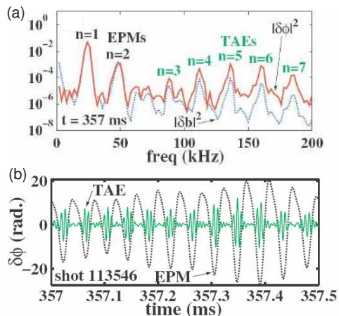
Figure 9: (a) Mirnov and reflectometer spectra showing multiple EPM and TAE modes, and (b) toroidal localization of TAE amplitude envelope from 3-wave coupling to n=1 EPM.
