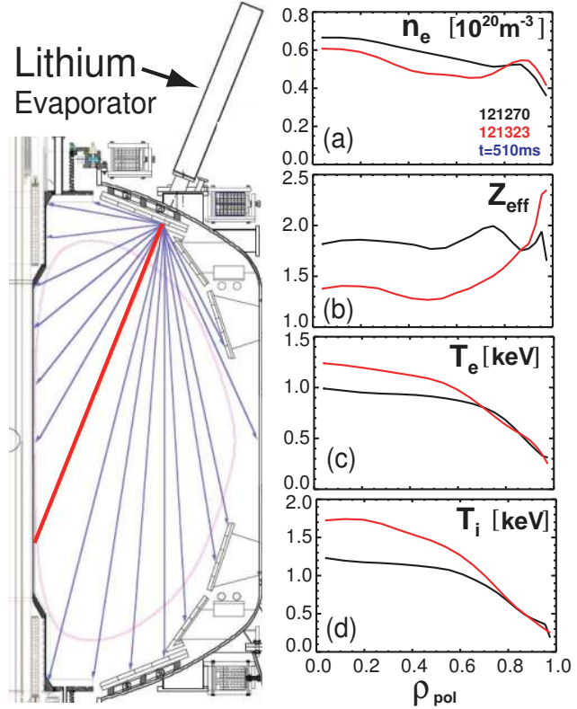
Figure 11: Comparisons of (a) n_e , (b) Z_{eff} , (c) T_e , and (d) T_i before (black) and after (red) lithium evaporation conditioning.
