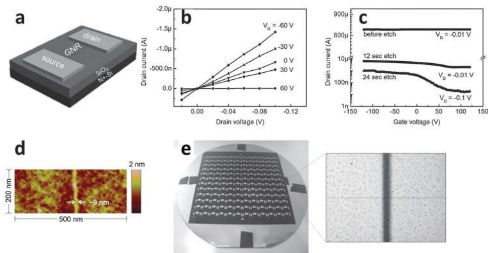
Fig. 16 (a) Architecture of a GNR-FET. (b) Output characteristics and (c) transfer characteristics of a GNR-FET. (d) AFM image of a 9 nm-wide GNR region. (e) Photograph of 144 GNR-FETs on a 4-inch wafer with the protective PVK NW not removed. (Reproduced with permission from ref. 145, Copyright 2014, Wiley-VCH Verlag GmbH & Co.)
