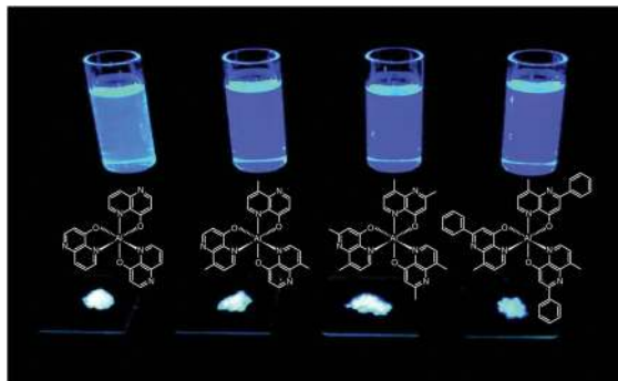
Fig. 5 Emission images of AlIND 3 , AlmND 3 23 , AlmmND 3 24 , and AlmpND 3 25 recorded in solution and solid state under irradiation by UV light. (Reproduced with permission from ref. 16. Copyright 2009, American Chemical Society.)
