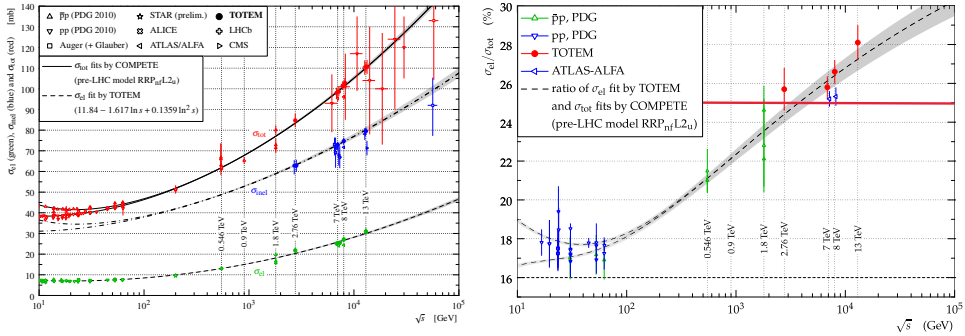
Figure 4. Left panel: The total, elastic and inelastic cross-sections as measured at various LHC energies and below. The total cross-section at \sqrt{s} = 13 TeV is determined with \rho = 0.1 at this energy. Overview of total ( \sigma_{tot} ), inelastic ( \sigma_{el} ) and elastic ( \sigma_{el} ) cross-sections for pp and p\bar{p} collisions as a function of \sqrt{s} , including TOTEM measurements over the whole energy range explored by the LHC. Uncertainty band on theoretical models and/or fits are described in the Legend. The continuous black lines (lower for pp , upper for p\bar{p} ) represent the best fits of the total cross section data by the COMPETE collaboration. The dashed line results from a fit of the elastic scattering data. The dash-dotted lines refer to the inelastic cross section and are obtained as the difference between the continuous and dashed fits. From refs. [1, 2]. Right panel: The elastic to total cross-section ratio increases with increasing energies, as indicated on this Figure from ref. [1]. At the LHC energies between 8 and 13 TeV it crosses significantly the important limit of (1 + \rho_0^2)\sigma_{el}/\sigma_{tot} = 1/4 . It is important to note that this ratio reaches the critical value in the region of \sqrt{s} = 2.76 - 7 TeV and it clearly exceeds it at \sqrt{s} = 13 TeV. The best COMPETE fit suggests a threshold behaviour in the region of \sqrt{s} = 2.76 - 4 TeV.
