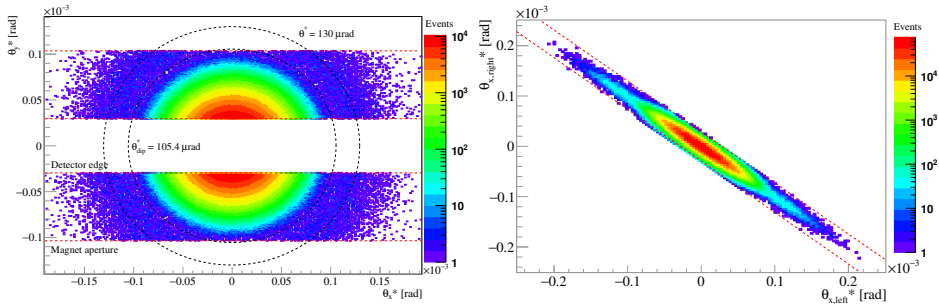
Figure 1. Left panel: Rotational symmetry of elastic scattering in the (\theta_x^*, \theta_y^*) plane at \sqrt{s} = 13 TeV proton-proton collisions, as measured by TOTEM and detailed in ref. [3]. The red dashed lines show the analysis acceptance cuts, which define the acceptance boundaries near the detector edge and magnet aperture. The inner black dashed circle illustrates the approximate scattering angle position \theta_{dip}^* = 105.4 \mu\text{rad} of the diffractive minimum, while the outer black dashed line indicates the approximate scattering angle position of \theta_{bump}^* = 130 \mu\text{rad} of the diffractive maximum. Right panel: Collinearity of the horizontal scattering angles at the collision point \theta_{x,left}^* and \theta_{x,right}^* in elastic pp scattering at \sqrt{s} = 13 TeV proton-proton collisions, as reconstructed by TOTEM [3]. The dotted lines indicates 4\sigma physics cuts applied to select the elastic events. See ref. [3] for the collinearity cuts on the vertical scattering angle \theta_y^* as well as further details on the other analysis cuts.
