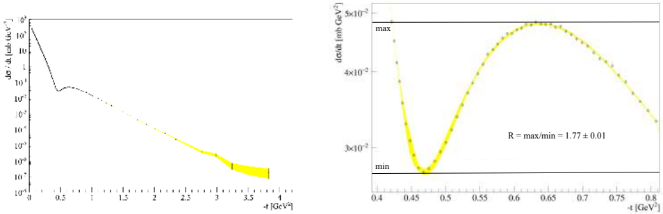
Figure 7. Left panel: TOTEM data for the differential cross-section of elastic pp scattering at \sqrt{s} = 13 TeV, from ref. [3]. The statistical and |t| -dependent correlated systematic uncertainty envelope is indicated by a yellow band. Right panel: The same TOTEM data for the differential cross-section of elastic pp scattering at \sqrt{s} = 13 TeV as on the left panel, but zooming in to the dip-and-bump region.
