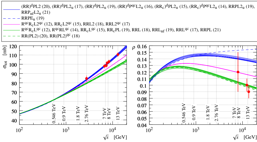
Figure 2. COMPETE bands for the total cross-section \sigma_{tot}(s) and the \rho(s) indicate [16] that without an Odderon contribution, recent TOTEM data at \sqrt{s} = 13 TeV for the pair of (\sigma_{tot}, \rho) cannot be described simultaneously.
