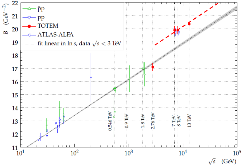
Figure 5. Excitation function of the slope parameter B in elastic proton-proton scattering. The TOTEM data at 2.76, 7, 8 and 13 TeV suggest the opening of a new channel between \sqrt{s} = 2.76 and 7 TeV, as noted in ref. [1] and indicated qualitatively by the red dashed line.
