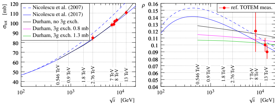
Figure 3. Measured values of \sigma_{tot} and \rho are compared to two different class of model calculations. The comparisons indicate that with an Odderon contribution, the recent TOTEM data for the pair of (\sigma_{tot}, \rho) at \sqrt{s} = 13 TeV can be described simultaneously: Predictions of the Odderon model by Nicolescu and collaborators are shown by a dashed [18] and solid blue curves [19]. Results from the KMR model [20] without Odderon effects are shown with a black line, and with Odderon effects are shown with magenta and green lines, where the crossing-odd contribution is taken from ref. [21]. Reference TOTEM measurements are indicated by red dots.
