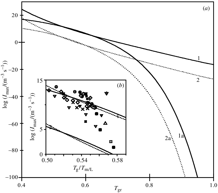
Figure 2. Maximum nucleation rate as a function of reduced glass-transition temperature. (a) The lines are calculated from the CNT with T_{0r} = 0.4 (1, 2) and C_2 = 4.5 (1a, 2a) for different thermodynamic barriers: C_1 = 5 (1, 1a), C_1 = 7 (2, 2a). (b) Points refer to experimental data. The lines are calculated from the CNT with C_1 = 4.5 (1), C_1 = 6.5 (2). Solid lines, C_2 = 4.5 and T_{0r} = T_{\text{gr}} - C_2/30 ; dashed lines, T_{0r} = 0.4 . (After Fokin et al. (2002a).)
