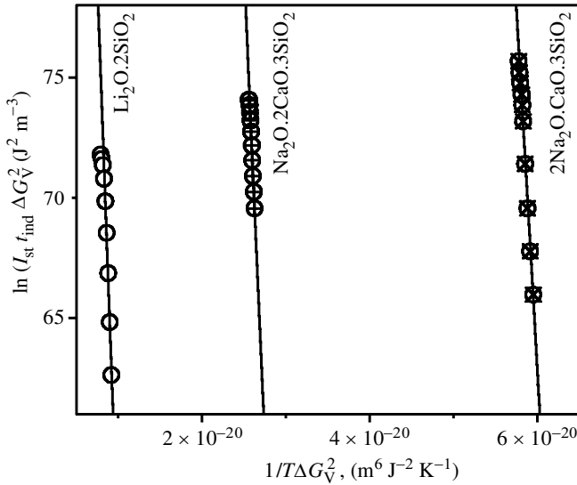
Figure 3. Plots of \ln(I_{\text{st}} t_{\text{ind}} \Delta G_v^2) against 1/T\Delta G_v^2 for three stoichiometric glasses. Linear fit for T > T_g . \Delta G_v corresponds to \Delta C_p = f(T) .
