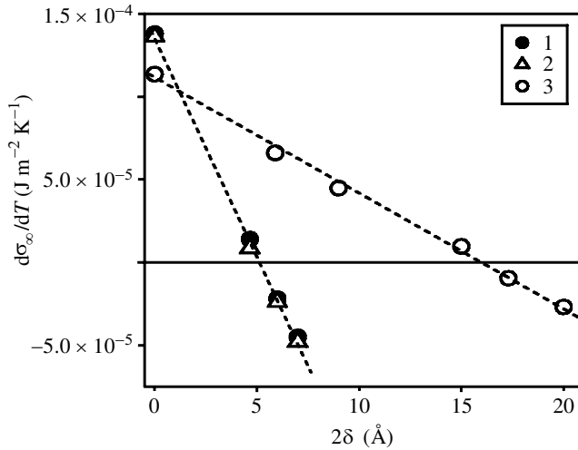
Figure 6. Average values of d\sigma_{\infty}/dT against Tolman's parameter for \text{Li}_2\text{O} \cdot 2\text{SiO}_2 (1, 2) and \text{Na}_2\text{O} \cdot 2\text{CaO} \cdot 3\text{SiO}_2 (3) crystals in parent glasses having the same compositions. The kinetic barrier for nucleation was estimated from time lag of nucleation (2, 3) and viscosity (1). (Reproduced with permission from Fokin & Zanotto (2000).)
