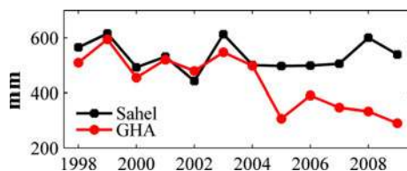
Fig. 3 Satellite-derived TRMM 3B43 mean regional JJAS precipitation totals within the GHA (red) and Sahel (black) from 1998 to 2009
