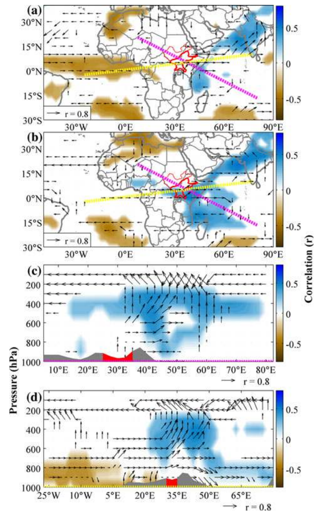
Fig. 7 Correlation between JJAS precipitation in the southern GHA and atmospheric circulation (including moisture transports) from 1948 to 1988 (NCEP/NCAR reanalysis). Only correlations exceeding the 90% significance level are shown. a Correlation with horizontal moisture transports ( arrows ) and specific humidity ( background ) within the lower troposphere below 700 hPa. b Correlation with horizontal wind velocity ( arrows ) and specific humidity ( background ) within the mid-troposphere between 700 and 500 hPa. c and d Vertical profiles of correlation with horizontal and vertical wind velocity ( arrows ) and specific humidity ( background ) along the transects defined by the pink ( c ) and yellow ( d ) dotted lines in a and b . Arrows in all plots represent correlation with velocity in zonal and meridional directions ( a and b ) or horizontal and vertical directions ( c and d ). Each arrow is the hypotenuse of an invisible triangle, of which the lengths of the x - and y -axes indicate the strength of correlation. Grey areas at the bottom of ( c ) and ( d ) represent land. Bold red outlines in a and b and red areas in c and d bound the southern GHA. Thin red outlines in a and b bound the rest of the GHA
