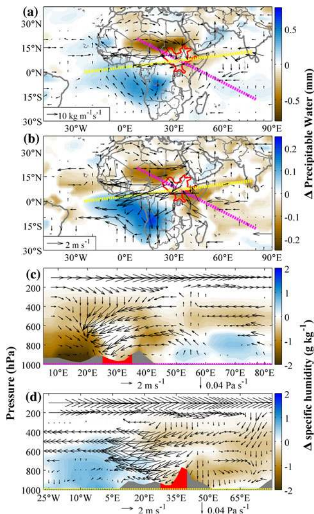
Fig. 18 Change in mean atmospheric circulation and moisture transports between the 1948–1988 period and the 1989–2009 period (NCEP/NCAR reanalysis). Only changes exceeding the 90% significance level according to a 2-tailed student's t test are shown. a Changes in horizontal moisture transports ( arrows ) and specific humidity ( background ) within the lower troposphere below 700 hPa. b Changes in horizontal wind velocity ( arrows ) and specific humidity ( background ) within the mid-troposphere between 700 and 500 hPa. c and d Vertical profiles of changes in horizontal and vertical wind velocity ( arrows ) and specific humidity ( background ) along the transects defined by the pink ( c ) and yellow ( d ) dotted lines in a and b . Grey areas at the bottom of ( c ) and ( d ) represent land. Bold red outlines in a and b and red areas in c and d represent the GHA
