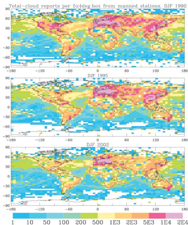
FIG. 3. Spatial distributions of the number of reports of total cloud cover per each 4° lat × 5° lon box from manned stations during December–February in (top) 1990, (middle) 1995, and (bottom) 2002. See Fig. 2 for data sources.
