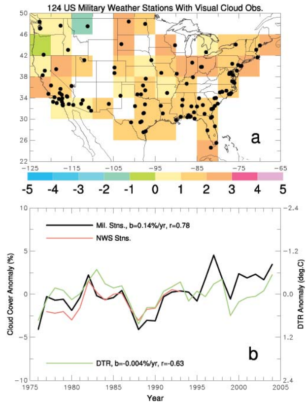
FIG. 8. (a) Distribution of 124 U.S. military weather stations (dots) with continuous human visual observations of total cloud cover, together with linear trends (color, percent sky per decade) of annual daytime total cloud cover during 1976–2004. (b) Anomaly time series of annual daytime total cloud cover averaged over the 4^{\circ} lat \times 5^{\circ} lon boxes that have at least one of the stations shown in (a) (black line, b is its slope and r is the correlation with the red line) and derived using all the NWS/FAA stations (red line, from 1976 to 1993 only). Also shown is the DTR anomaly (green line, decreases downward on the right-side ordinate, b is its slope and r is the correlation with the black line) averaged over the same areas with data in (a) using the updated GHCN v2 dataset (Peterson and Vose 1997).
