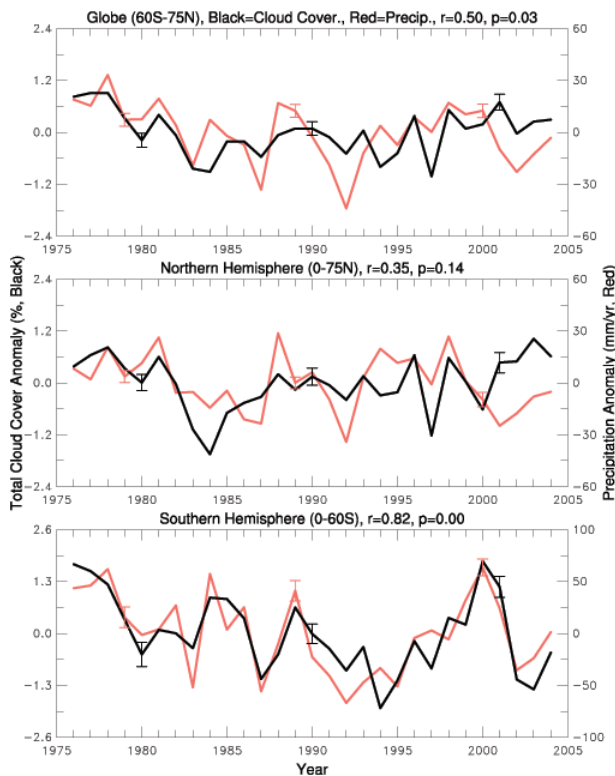
FIG. 1. Comparison of annual total cloud cover (black) and precipitation (red) averaged over the same land areas of the globe (60°S–75°N), Northern Hemisphere (0°–75°N), and Southern Hemisphere (0°–60°S), excluding the United States and Canada (because of the ASOS-induced discontinuity over these two countries). The cloud cover was derived using surface observations from over 15,000 weather stations (the GTS data archived at NCAR, see information online at http://dss.ucar.edu/datasets/ds464.0/ ). The station data were first arithmetically averaged within each 1° × 1° box and then the 1° anomalies were further averaged onto a 4° lat × 5° lon grid, on which the regional mean was derived using area-weighted averaging. Precipitation data are from Chen et al. (2002 and updates). The error bars represent ± one standard error estimated using the inter-grid-box variations.
