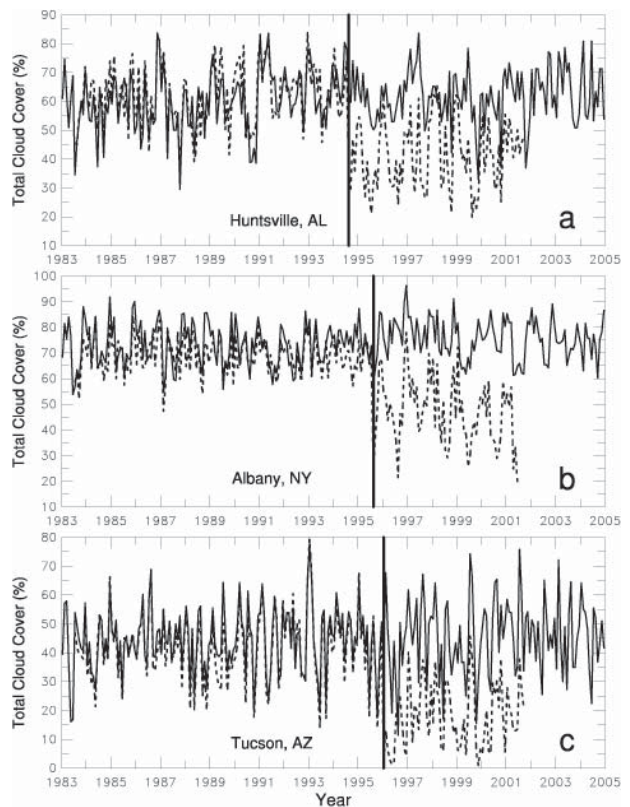
FIG. 4. Time series of monthly mean daytime total cloud cover (dashed line) from three NWS/FAA stations at (a) Huntsville, AL, (b) Albany, NY, and (c) Tucson, AZ. The vertical line indicates the time when the ASOS was introduced. Also shown are human visual observations of daytime total cloud cover from a closest military weather station (solid line).
