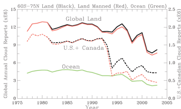
FIG. 2. Annual number of reports of total cloud cover from manned (red) and automated plus manned (black) stations from global land (upper curves), the United States and Canada (middle dashed curves, scales on the right side) (from the GTS data archived at NCAR, see information online at http://dss.ucar.edu/datasets/ds464.0/ ), and global oceans [green, all reports, from the International Comprehensive Ocean–Atmosphere Data Set (ICODAS) information online at www.cdc.noaa.gov/coads/ ]. Units: millions.
