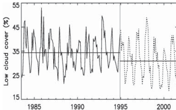
FIG. 5. Monthly time series of daytime low cloud cover (with cloud-base height below 2 km) over the contiguous United States from surface visual (black solid line) and ASOS (dashed line) observations (see Sun and Groisman 2004 for more details about the data). The mean for the visual and ASOS observations are 34.4% and 30.9%, respectively, as indicated by the horizontal lines.
