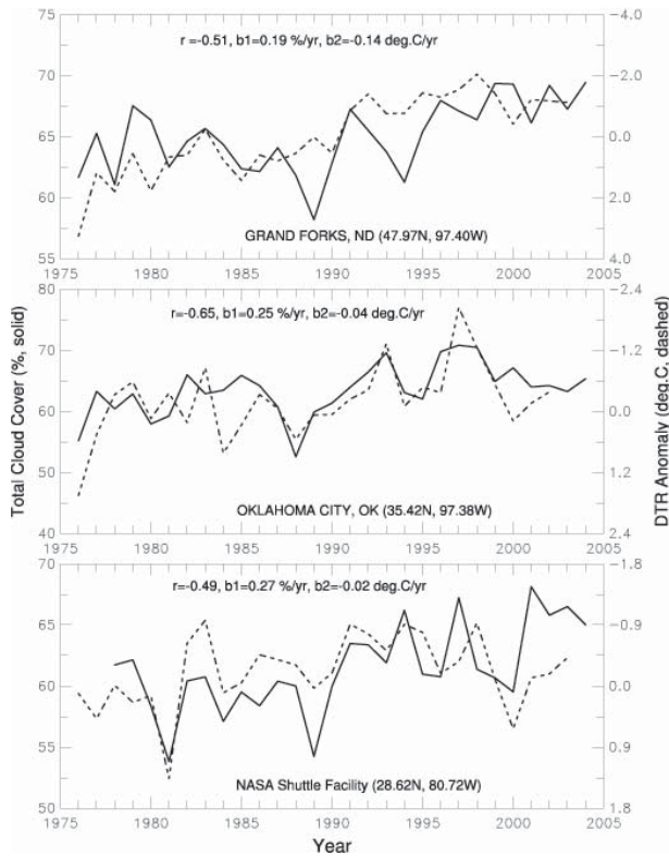
FIG. 7. Time series of annual mean daytime (0600–1800 local solar time) total cloud cover (percent of the sky, solid line) at three U.S. military weather stations, compared with the annual mean DTR anomaly ( ^{\circ}\text{C} , dashed line, increases downward on the right-side ordinate) from a nearby synoptic weather station. Also shown are the correlation coefficient ( r ) between the two curves and the slope of the curves ( b_1 for cloud cover and b_2 for DTR). The station DTR data were extracted from the updated GHCN v2 dataset (Peterson and Vose 1997).
