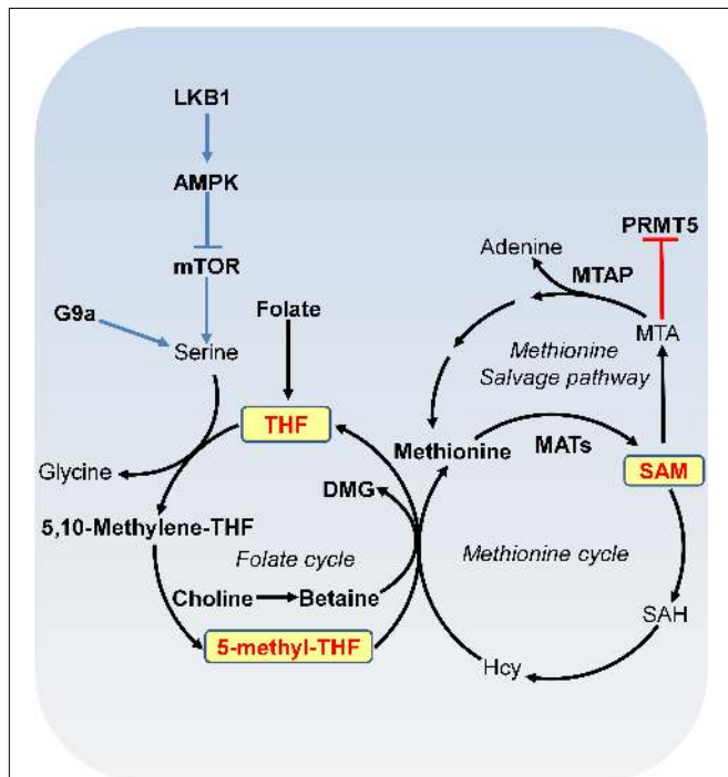
FIGURE 2 | Metabolism of SAM. SAM is synthesized from methionine and ATP by methionine adenosyltransferase (MAT). In methylation reactions, SAM is sequentially converted to S-adenosylhomocysteine (SAH), homocysteine (Hcy) and methionine with 5-methyl-tetrahydrofolate (THF) or with betaine as the methyl donor. Serine-glycine metabolism provides one-carbon unit to the folate cycle. Serine biosynthesis is controlled by LKB-AMPK-mTOR pathway. In the methionine salvage pathway, SAM is converted to 5'-methylthioadenosine (MTA), which is salvaged back for SAM generation. MTA inhibits the activity of PRMT5. MAT, methionine adenosyltransferase; MTA, 5'-methylthioadenosine; THF, tetrafolate; LKB1, liver kinase B1; mTOR, mammalian target of rapamycin complex; SAH, S-adenosylhomocysteine; Hcy, homocysteine; MTAP, MTA phosphorylase; DMG, dimethylglycine; PRMT5, arginine methyltransferase 5.
