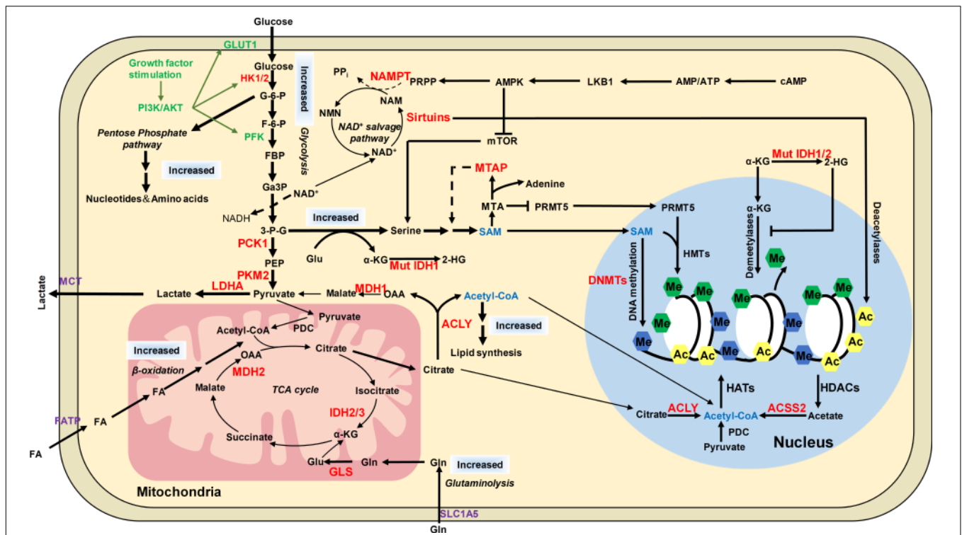
FIGURE 5 | The distinct metabolic pathways in cancer cells and their connection to epigenetic modifications. Cancer cells have increased glucose and glutamine uptake, leading to accelerated glycolysis and biomass accumulation. PI3K/AKT is activated by growth factors to regulate glycolysis and acetyl-CoA generation. AKT induces the expression of GLUT1 to increase glucose uptake and phosphorylates HK1 and PFK to enhance aerobic glycolysis. AKT phosphorylates ACLY to increase acetyl-CoA production. Increased lactate dehydrogenase (LDH) activity and decreased pyruvate dehydrogenase (PDC) activity result in increased lactate export, attenuated TCA cycle and diversion of glycolysis to pentose phosphate pathway. ACLY, ACSS2 and PDC contribute to nuclear acetyl-CoA production and subsequent histone acetylation. Glycolysis is increased in cancer cells with NAD + converted to NADH, leading to reduced NAD + /NADH ratio and downregulated activity of sirtuins, which results in histone hyperacetylation and dysregulation of gene expression. Serine and one-carbon metabolism is also accelerated in cancer cells to produce SAM, which is controlled by LKB-AMPK-mTOR pathway. α-KG is primarily produced by transamination of glutamate derived from glutamine in cancer cells. Mutations of IDH1/2 lead to accumulation of 2-HG, which increases histone methylation by inhibiting α-KG dependent enzymes. The potential targets for anti-cancer therapy were labeled in red color. ACSS2, acetyl-CoA synthetase short chain family member 2; AMPK, AMP-activated protein kinase; F-6-P, fructose-6-phosphate; FBP, fructose-1,6-bisphosphate; GA3P, glyceraldehyde-3-phosphate; Gln, glutamine; Glu, glutamate; HK1/2, hexokinase 1/2; LDHA, lactate dehydrogenase; MCT1, monocarboxylate transporter 1; MCT4, monocarboxylate transporter 4; MDH1, malate dehydrogenase 1; Mut IDH1/2, mutated isocitrate dehydrogenase 1 and 2; MTA, 5'-methylthioadenosine; MTAP, MTA phosphorylase; NAM, nicotinamide; NAMPT, nicotinamide phosphoribosyltransferase; NMNATs, nicotinamide mononucleotide adenylyltransferases; PCK1, phosphoenolpyruvate carboxykinase 1; PDC, pyruvate dehydrogenase complex; PEP, phosphoenolpyruvate; PFK, phosphofructokinase; PI3K, phosphoinositide 3-kinase; PKM2, pyruvate kinase M2; PRMT5, arginine methyltransferase 5; PRPP, phosphoribosyl pyrophosphate; α-KG, α-ketoglutarate; 2-HG, 2-hydroxyglutarate; 3-P-G, 3-phosphoglycerate; ACLY, ATP-citrate lyase.
