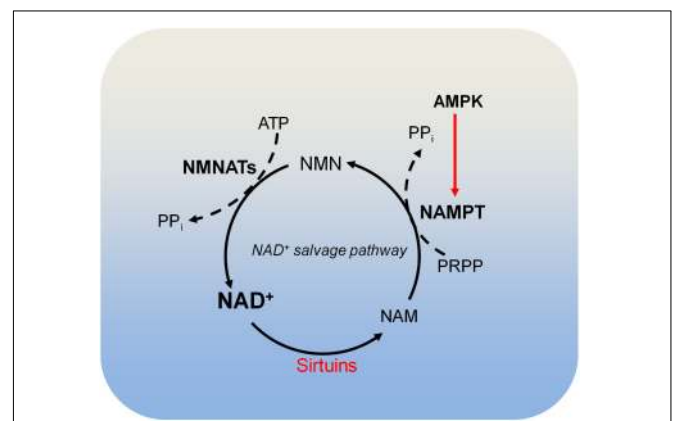
FIGURE 4 | Metabolism of NAD + . Sirtuins consume NAD + and produce nicotinamide (NAM). NAM is recycled to produce NAD + by the NAD + salvage pathway. In the NAD + salvage pathway, NAM is converted to nicotinamide mononucleotide (NMN) by nicotinamide phosphoribosyltransferase (NAMPT), and NMN is then converted to NAD + by nicotinamide mononucleotide adenylyltransferases (NMNATs). AMPK is required for NAMPT expression and thus controls intracellular NAD + . NAM, nicotinamide; NAMPT, nicotinamide phosphoribosyltransferase; NMNATs, nicotinamide mononucleotide adenylyltransferases; PRPP, phosphoribosyl pyrophosphate.
