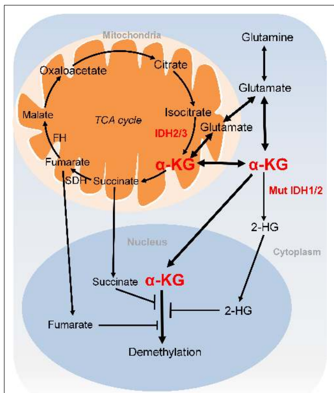
FIGURE 3 | Metabolism of α-KG. α-KG is synthesized from the TCA cycle or transamination of glutamate derived from glutamine. α-KG can be metabolized to succinate and fumarate in the TCA cycle. Succinate and fumarate are competitive inhibitors of α-KG-dependent demethylases. α-KG can also be converted to 2-HG by mutated isocitrate dehydrogenase 1 and 2 (IDH1 and IDH2). 2-HG is a competitive inhibitor of α-KG-dependent demethylases. α-KG, α-ketoglutarate; 2-HG, 2-hydroxyglutarate; Mut IDH1/2, mutated isocitrate dehydrogenase 1 and 2.
