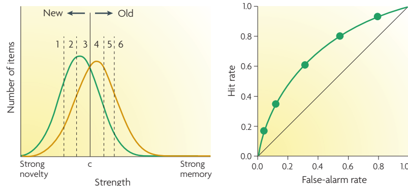
Figure 1 | Signal-detection theory and the receiver operating characteristic. a | The signal-detection representation 128 of a strong memory condition. The targets (old items) and foils (new items) in a recognition memory test are presumed to have varying degrees of memory strength (the subjective certainty that an item was or was not previously presented), and the mean and variance of the target distribution are greater than those of the foil distribution. A test item that generates a memory strength that exceeds a criterion value (indicated by the vertical line labelled c ) is declared to be 'old'. Otherwise, the test item is declared to be 'new'. Confidence ratings (indicated by vertical dashed lines) of one to six range from 'sure new' to 'sure old'. Items with memory strength to the left of the left-most vertical line are given 'high confidence new' responses. Items with memory strength to the right of the right-most vertical line are given 'high confidence old' responses. The right-hand panel shows a receiver operating characteristic (ROC) curve constructed from a subject's confidence ratings. Five pairs of hit and false-alarm rates are computed from the six-point confidence rating scale. The left-most point represents the hit and false-alarm rates for targets and foils that receive a rating of 6. The second point represents the proportion of targets and foils that receive a rating of either 5 or 6, and so on. As is almost always the case in strong memory conditions 129 , the resulting ROC curve in this example is asymmetrical. b | The signal-detection representation of a weak memory condition, in which the means and variances of the target and foil distributions are more similar and the ROC curve is more symmetrical.
