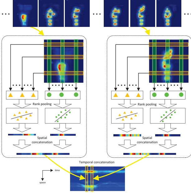
Figure 4: Generation of body shape evolution image via proposed spatial rank pooling
