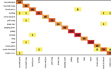
Figure 10: Confusion matrix of our method on PennAction dataset
