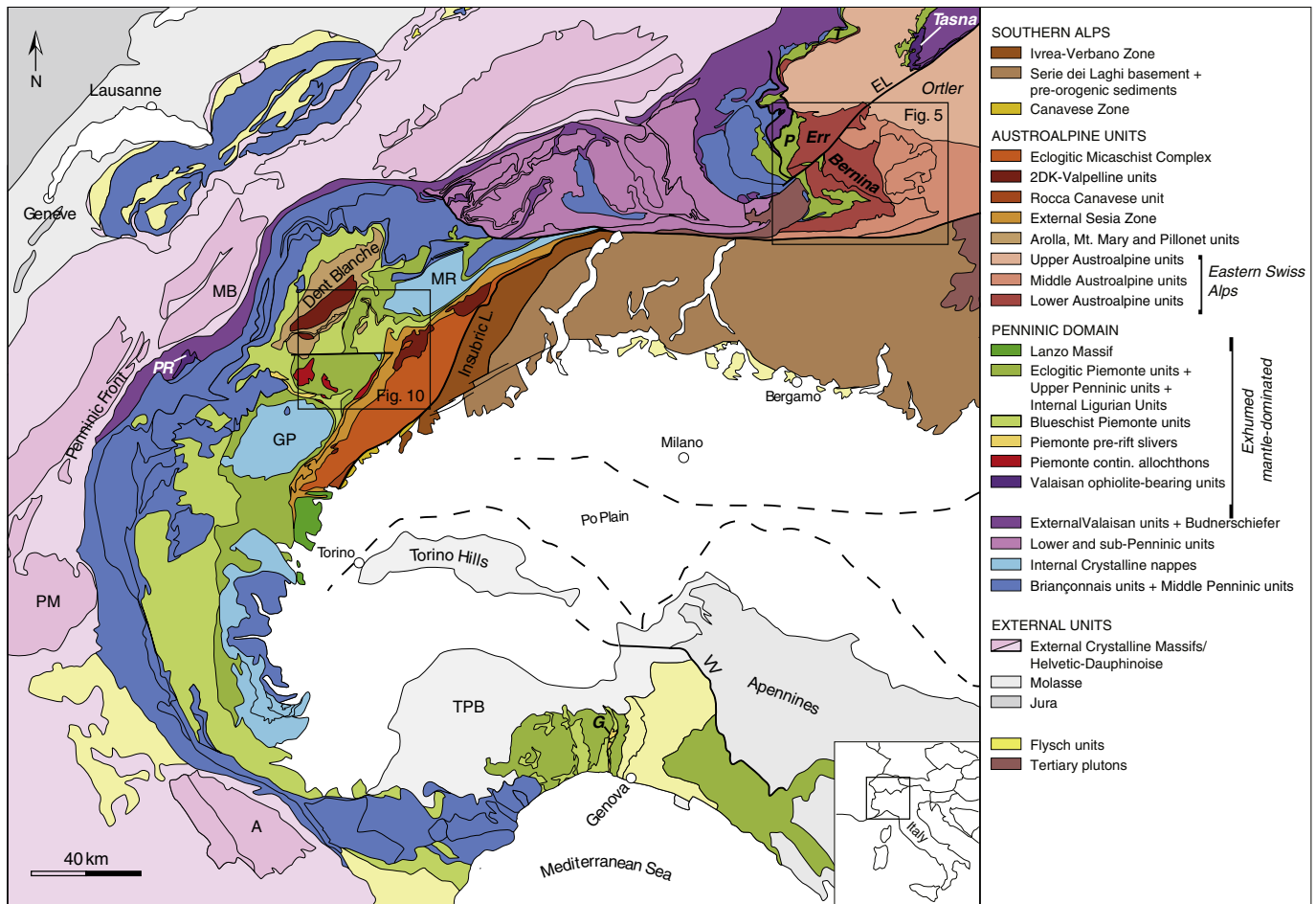
Fig. 4. Tectonic map of the Alps, compiled after Bigi et al., 1990; Handy et al., 1999; Capponi and Crispini, 2008; Bousquet et al., 2008; Molli et al., 2010; Galli et al., 2011; Mohn et al., 2011; Galster et al., 2012 and own observations. A: Argentera massif; G: Gazzo–Isoverde unit; GP: Gran Paradiso unit; MB: Mont Blanc massif; MR: Monte Rosa unit; P: Platta unit; PM: Pelvoux massif; PR: Punta Rossa unit; TPB: Tertiary Piemonte basin; VV: Villavernia–Varzi Line.
