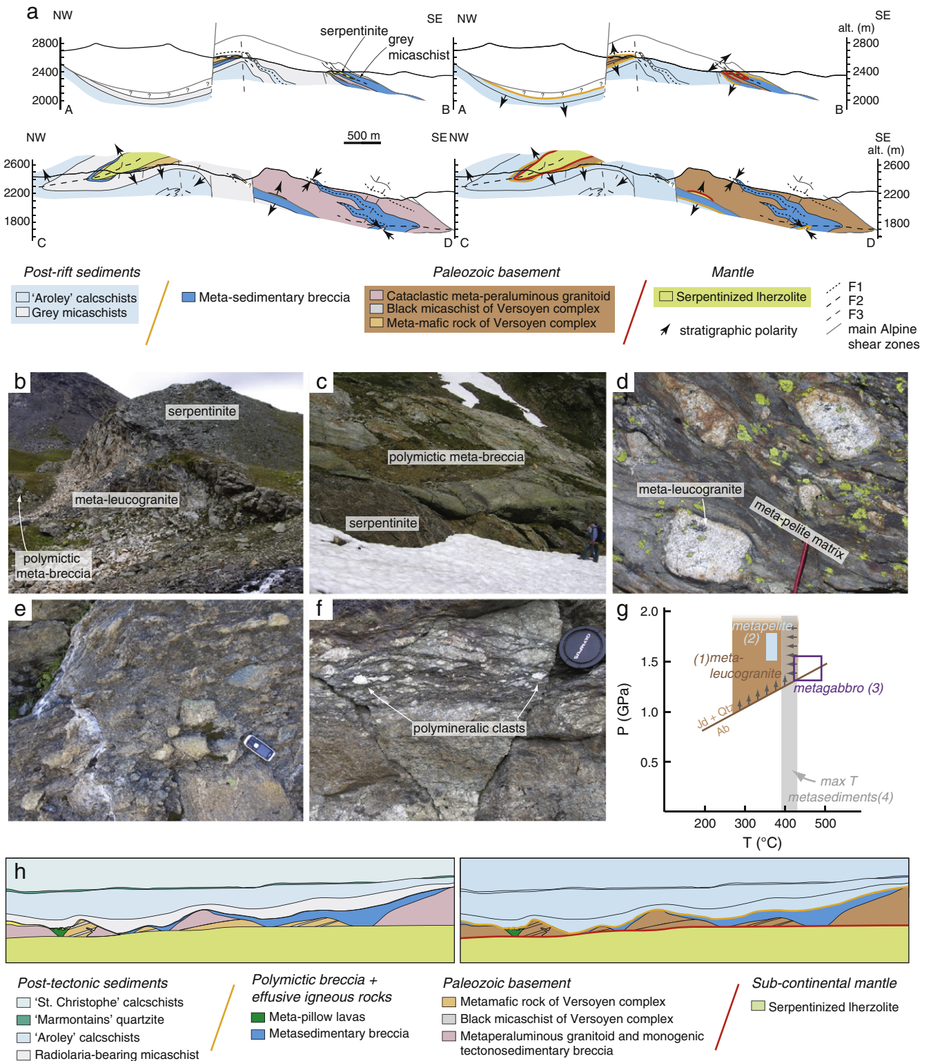
Fig. 9. Punta Rossa unit (Valaisan units). (a) Geological cross sections (modified after Beltrando et al., 2012). Note that basement allochthons consist of different rock types and that allochthons and coarse clastics, of presumed syn-tectonic deposition, are laterally discontinuous. If lithological differences in basement are discarded and key horizons identified, the large scale folds are more easily identified. In the Punta Rossa unit, serpentinitized mantle peridotites are directly in contact with Paleozoic basement, including meta-leucogranites (b; UTM WGS84 32N: 332734E; 5064201N) or polymictic breccias (c; UTM WGS84 32N: 333393E; 5062515N). Clasts of leucogranites are found occasionally in the post-tectonic gray micaschists (d; UTM WGS84 32N: 333563E; 5062645N) Monomictic breccias developed at the expense of serpentinitized peridotites (e; UTM WGS84 32N: 333324E; 5062516N) and meta-leucogranites (f; note the angular polymineralic clasts; UTM WGS84 32N: 332687E; 5064217N) can be interpreted as pre-metamorphic fault rocks. Estimates of the PT evolution of the different lithologies are hampered by extensive late-stage re-equilibration at greenschist facies conditions. Despite these limitations, all lithologies preserve evidence of metamorphic re-equilibration at P > 1.0 GPa (g). The maximum P estimated from meta-gabbros in the neighboring Hermite unit are also indicated. References: 1 = Saliot, 1979; 2 = Bousquet et al., 2002; 3 = Cannic et al., 1996; 4 = Beltrando et al., 2012. All these observations allow retro-deforming the present-day Punta Rossa unit into a pre-orogenic scenario (h). Retro-deformation is performed using the red and orange lines as markers.
