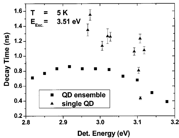
FIG. 3. Spectral dependence of time constants for single QD lines (triangles) and the QD ensemble (squares).
