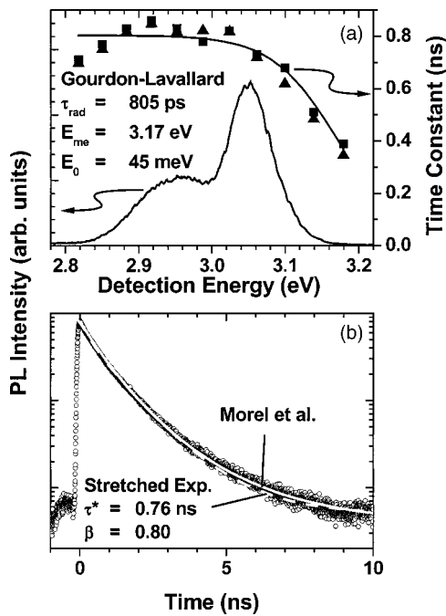
FIG. 1. (a) Time-integrated ensemble PL, time constant \tau_e of the 1/e decay (squares) and the fitting parameter \tau^* (triangles), fit with Eq. (2) (solid line). (b) Time-resolved ensemble PL, Fits with Eq. (1) (dashed line) and Morel et al. (Ref. 5) (solid line).
