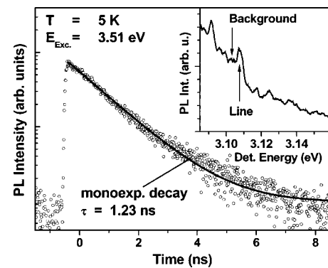
FIG. 2. Time-resolved PL of a single QD emission line (inset), fitted by a monoexponential decay (solid line).
