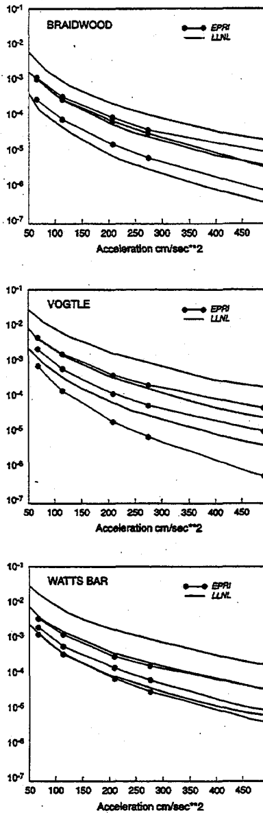
FIGURE 1.1 Median, 15th, and 85th percentile hazard curves for three representative separated sites in the eastern United States, illustrating the differences in results of the LLNL and EPRI studies. The ordinate is the estimated annual frequency of exceedance of the peak ground acceleration shown as the abscissae (adapted from Figures 2.3.1, 2.3.7, 2.3.8 in Bernreuter et al., 1987).
