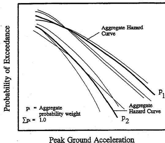
Figure 7-8 Illustration of an aggregate set of seismic hazard curves for PGA for soil site conditions. Each curve has an assigned weight to it.
