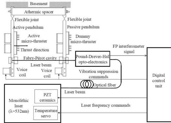
Figure 4. Example of a state-of-the-art hanging pendulum thrust stand. 38
